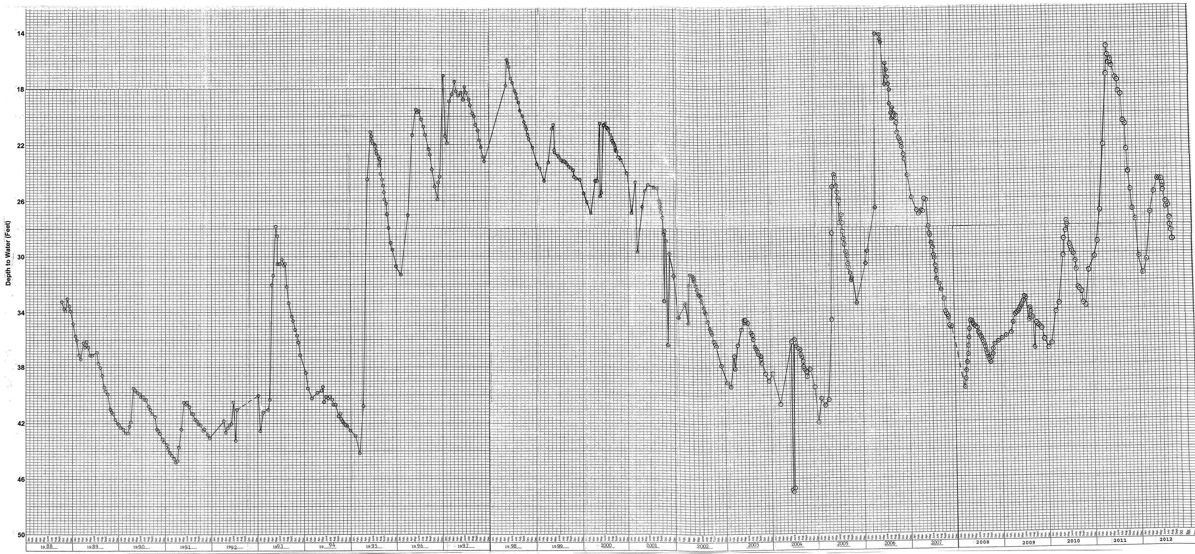
WATER-LEVEL HYDROGRAPH FOR WELL NO. 4M
