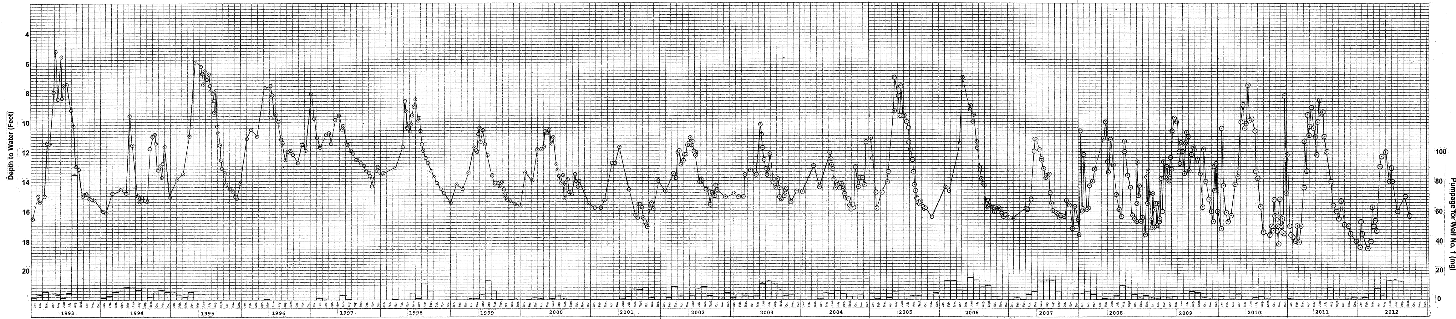
FIGURE 16-WATER-LEVEL HYDROGRAPH FOR WELL NO. 23 AND PUMPAGE FOR WELL NO. 1
