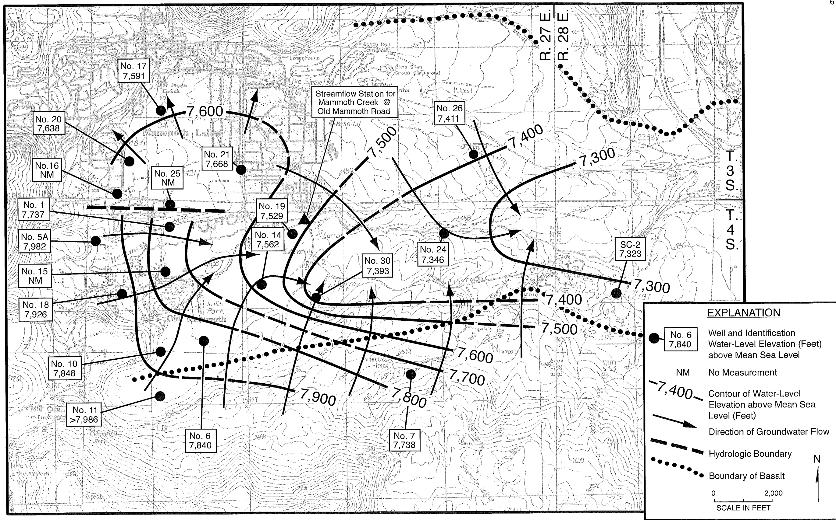
FIGURE 18 - WATER-LEVEL ELEVATIONS IN SEPTEMBER 2012
