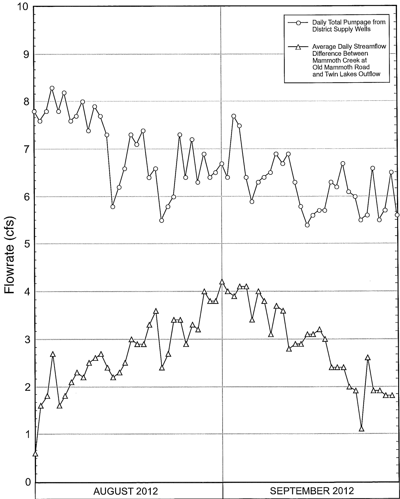
FIGURE 19 - RELATIONSHIP BETWEEN MAMMOTH CREEK STREAMFLOW DIFFERENCE AND DISTRICT PUMPAGE (AUGUST-SEPTEMBER 2012)
