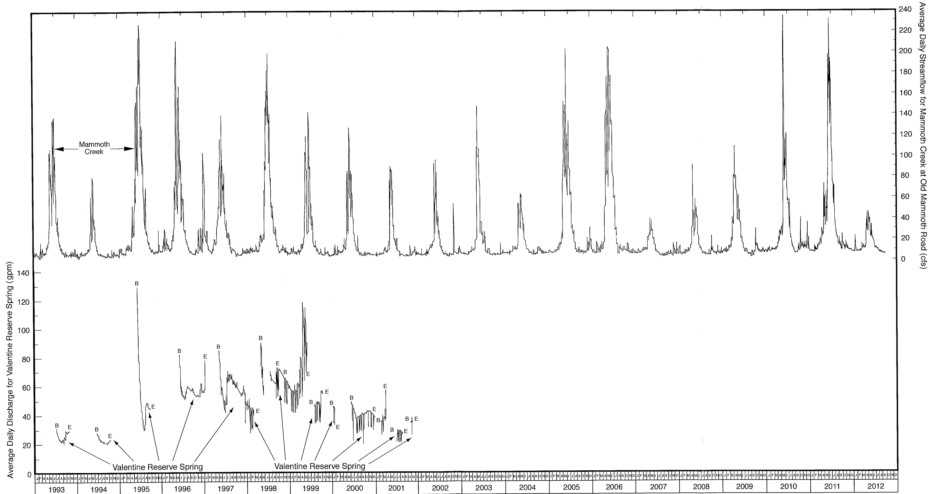
FIGURE 20 - FLOW FOR VALENTINE SPRING (1993-2001) AND MAMMOTH CREEK STREAMFLOW (1993-2012)
