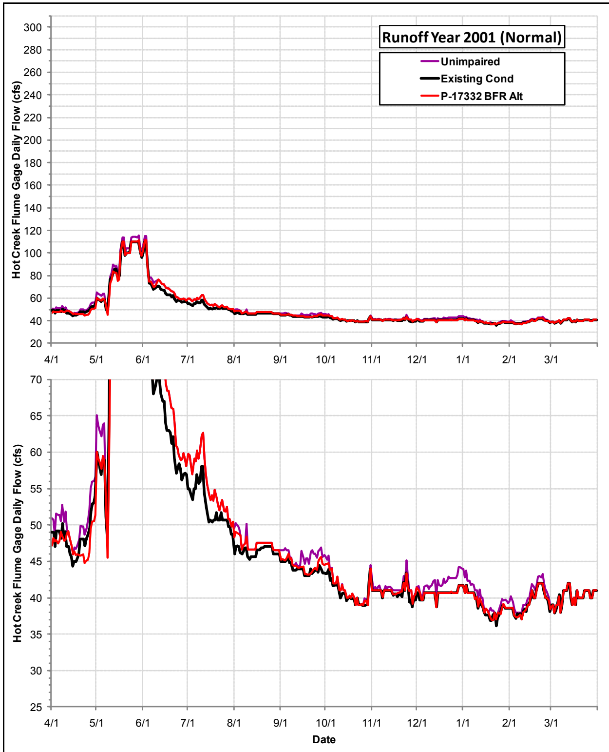
Daily Flows (cfs) at the USGS Hot Creek Flume Gage under the Permit 17332 Bypass Flow Requirements Alternative, the Existing Condition and the Index of Unimpaired Conditions during Runoff Year 2001
