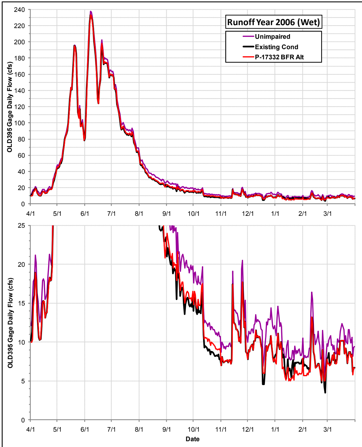
Daily Flows (cfs) at the OLD395 Gage under the Permit 17332 Bypass Flow Requirements Alternative, the Existing Condition and the Index of Unimpaired Conditions during Runoff Year 2006
