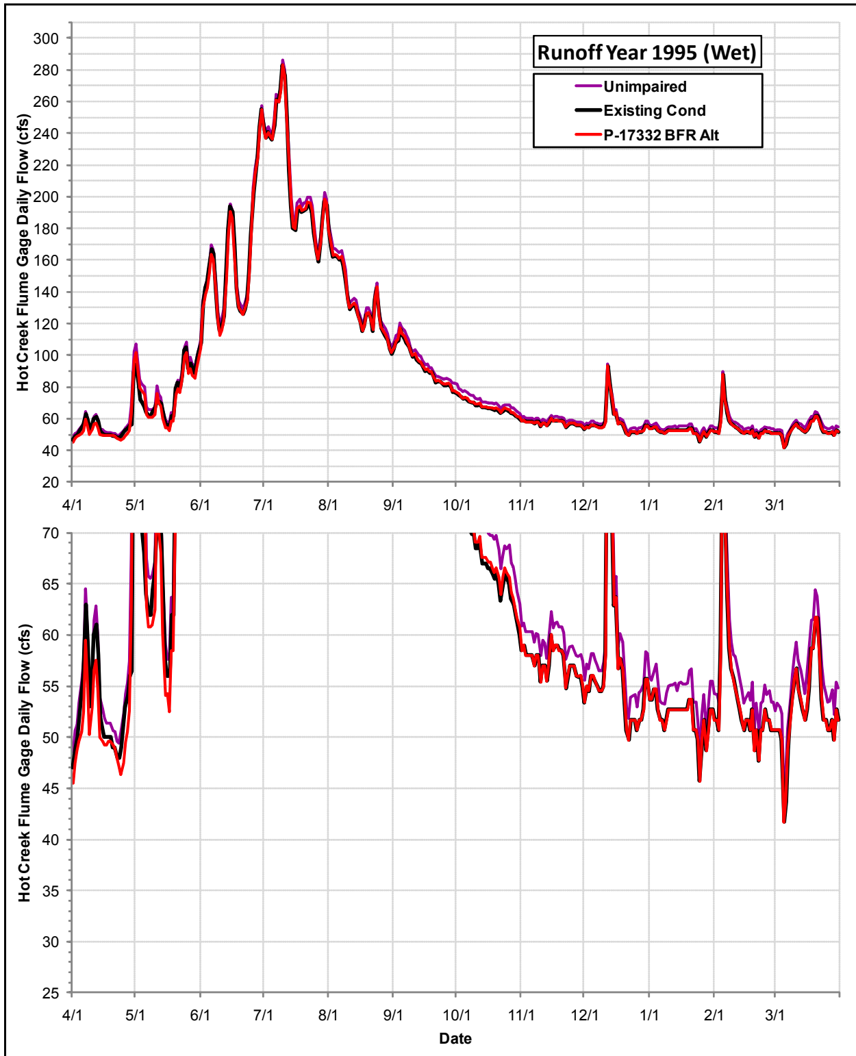
Daily Flows (cfs) at the USGS Hot Creek Flume Gage under the Permit 17332 Bypass Flow Requirements Alternative, the Existing Condition and the Index of Unimpaired Conditions during Runoff Year 1995
