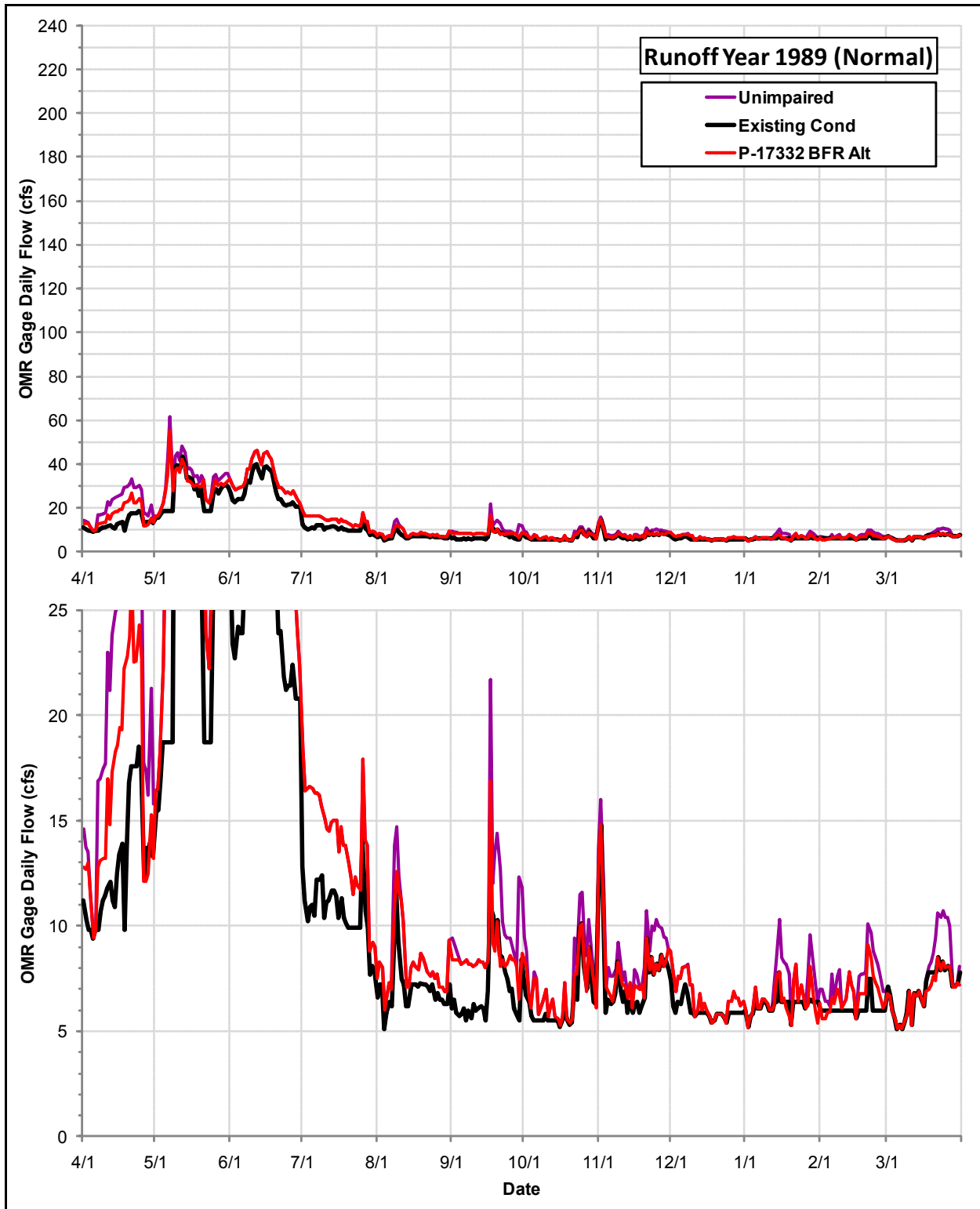
Daily Flows (cfs) at the OMR Gage under the Permit 17332 Bypass Flow Requirements Alternative, the Existing Condition and the Index of Unimpaired Conditions during Runoff Year 1989
