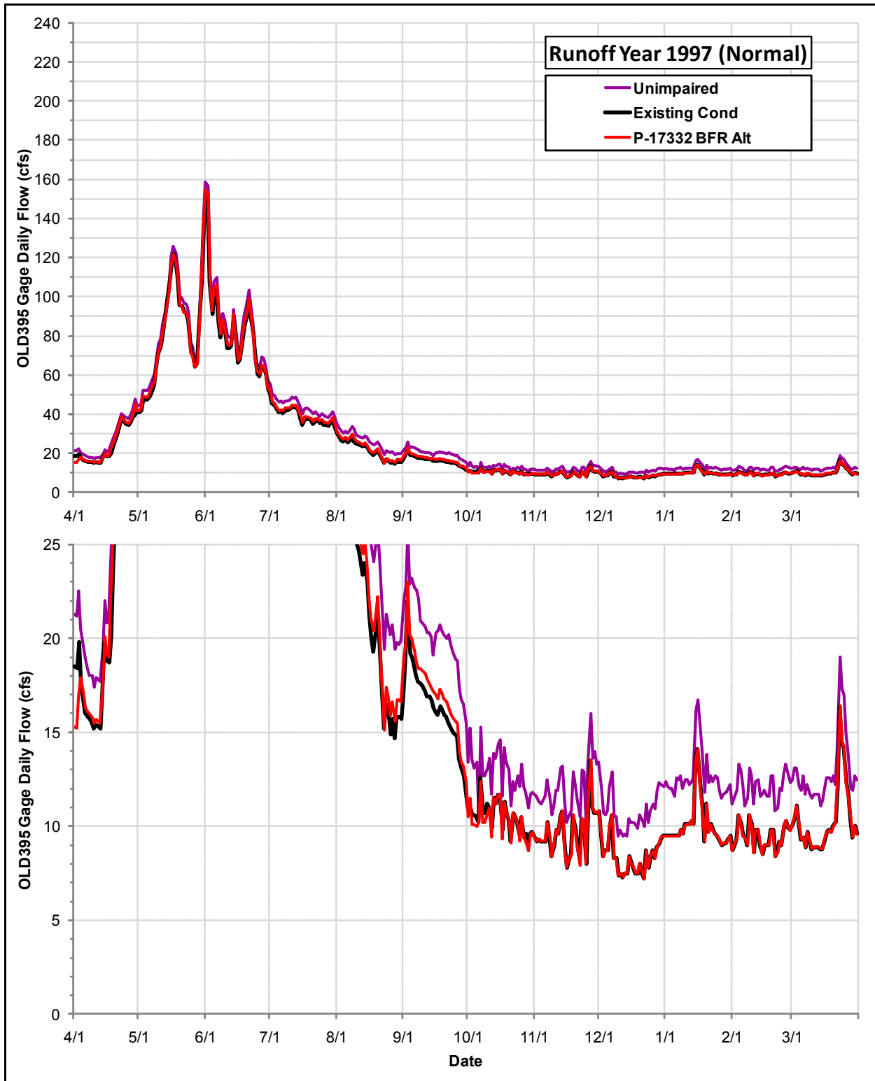
Daily Flows (cfs) at the OLD395 Gage under the Permit 17332 Bypass Flow Requirements Alternative, the Existing Condition and the Index of Unimpaired Conditions during Runoff Year 1997
