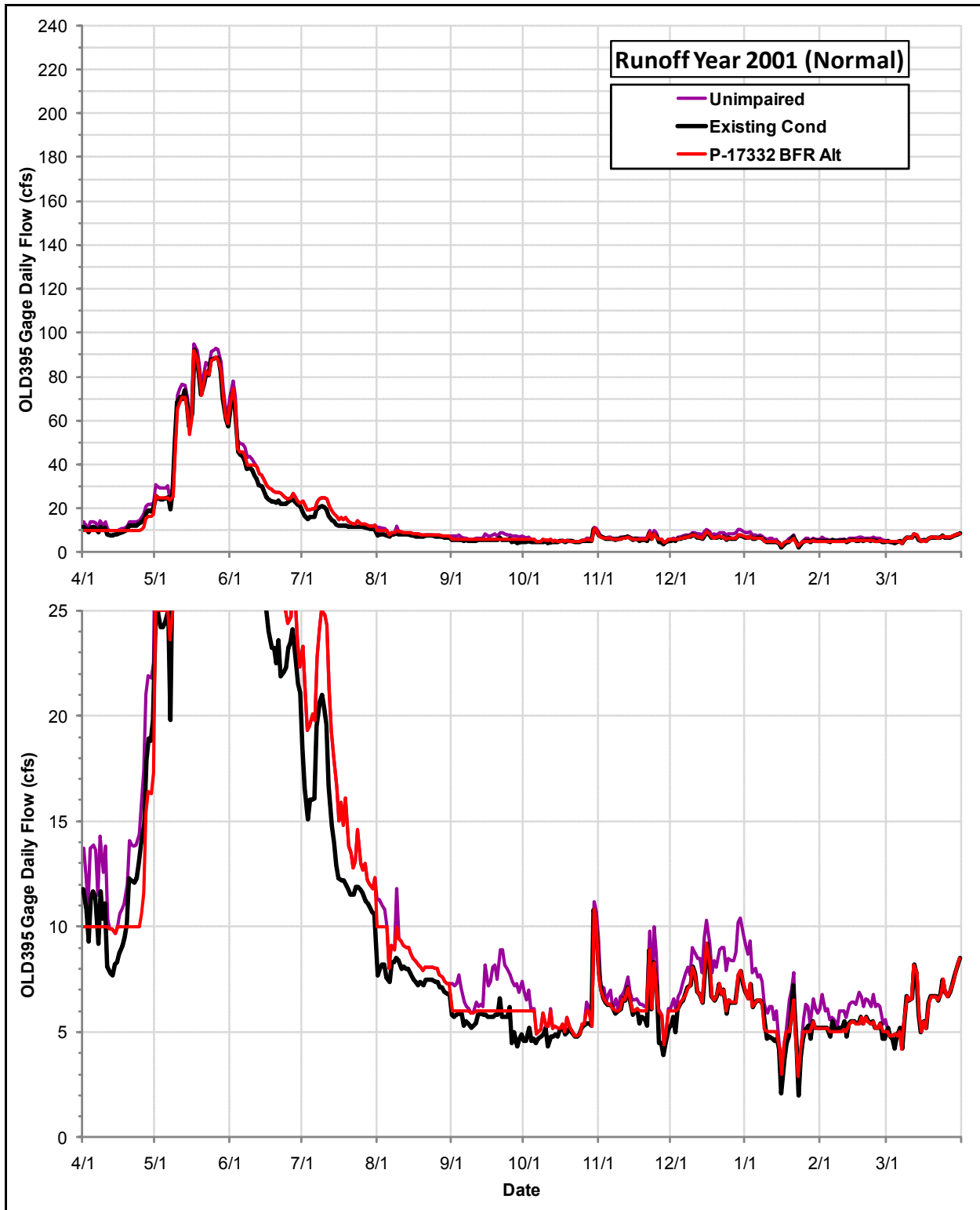
Daily Flows (cfs) at the OLD395 Gage under the Permit 17332 Bypass Flow Requirements Alternative, the Existing Condition and the Index of Unimpaired Conditions during Runoff Year 2001
