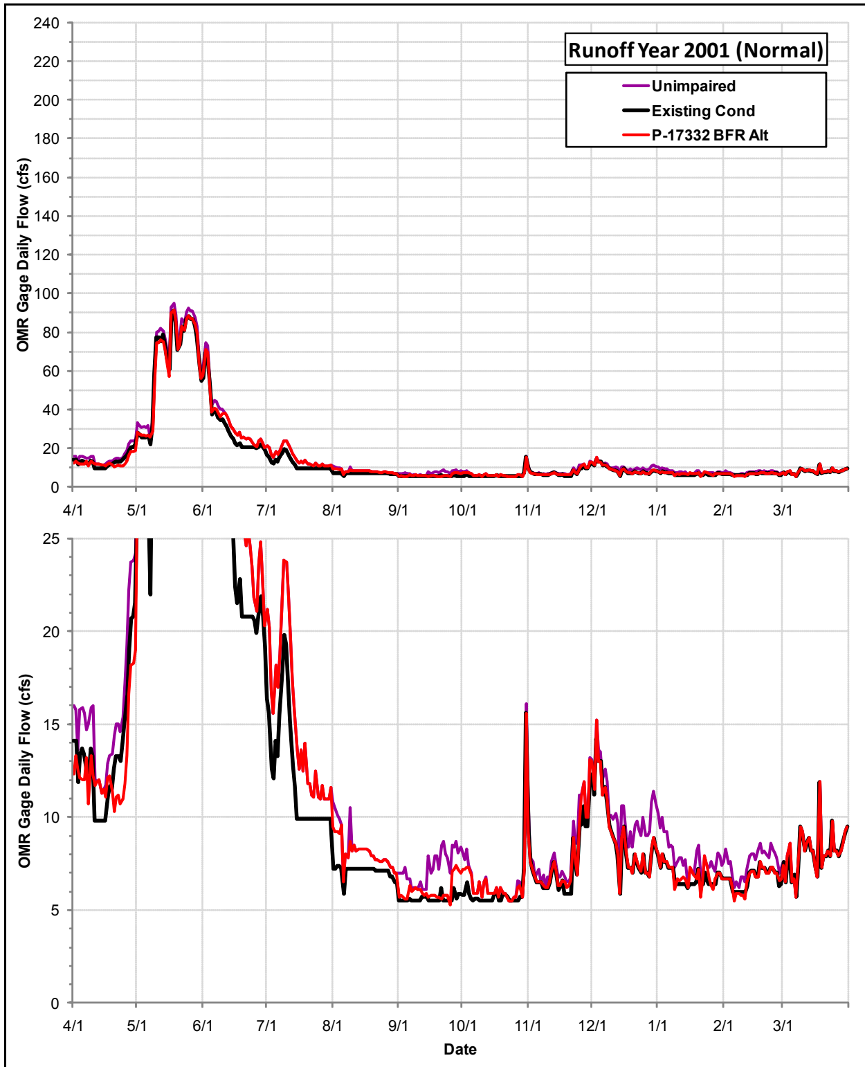
Daily Flows (cfs) at the OMR Gage under the Permit 17332 Bypass Flow Requirements Alternative, the Existing Condition and the Index of Unimpaired Conditions during Runoff Year 2001
