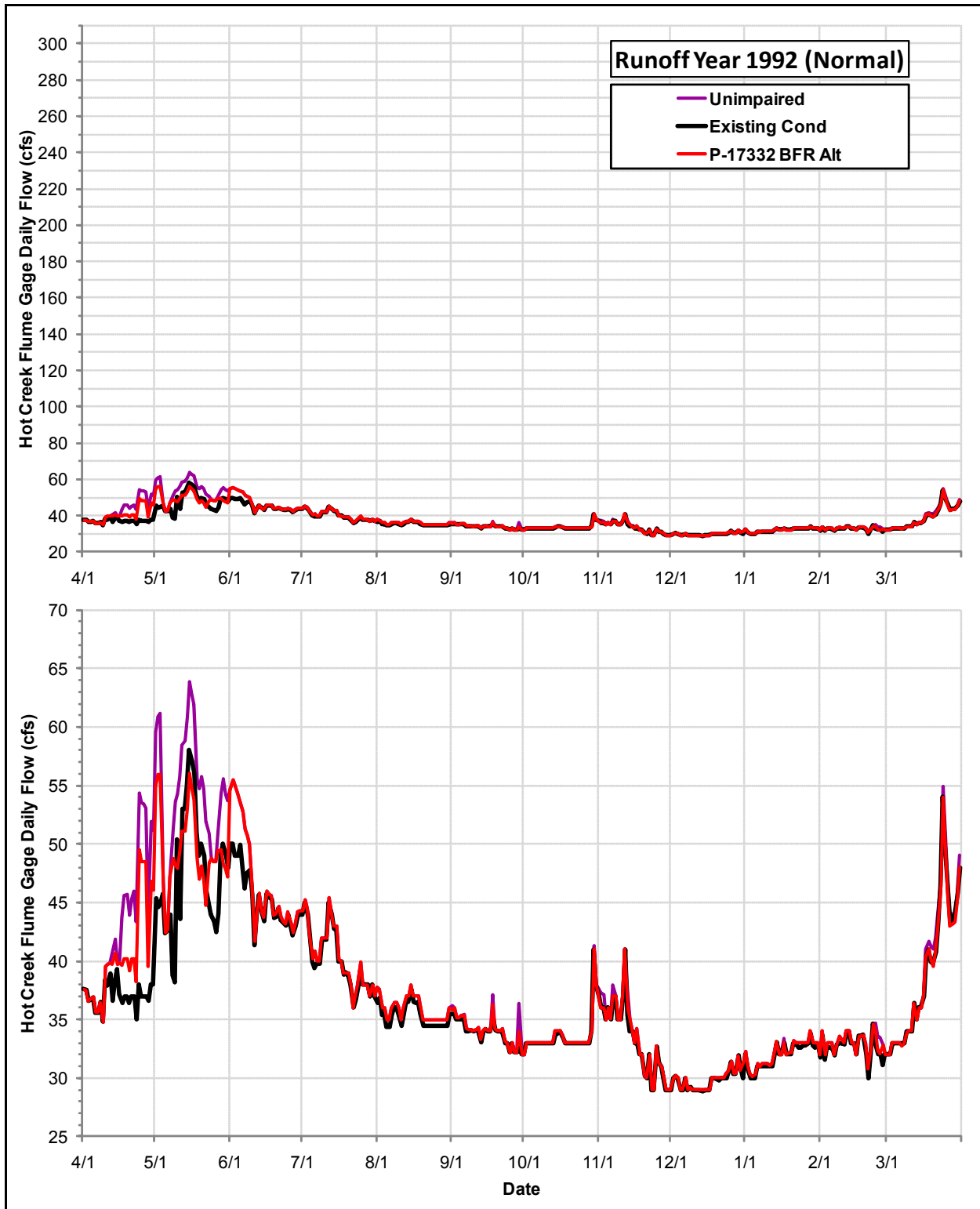
Daily Flows (cfs) at the USGS Hot Creek Flume Gage under the Permit 17332 Bypass Flow Requirements Alternative, the Existing Condition and the Index of Unimpaired Conditions during Runoff Year 1992
