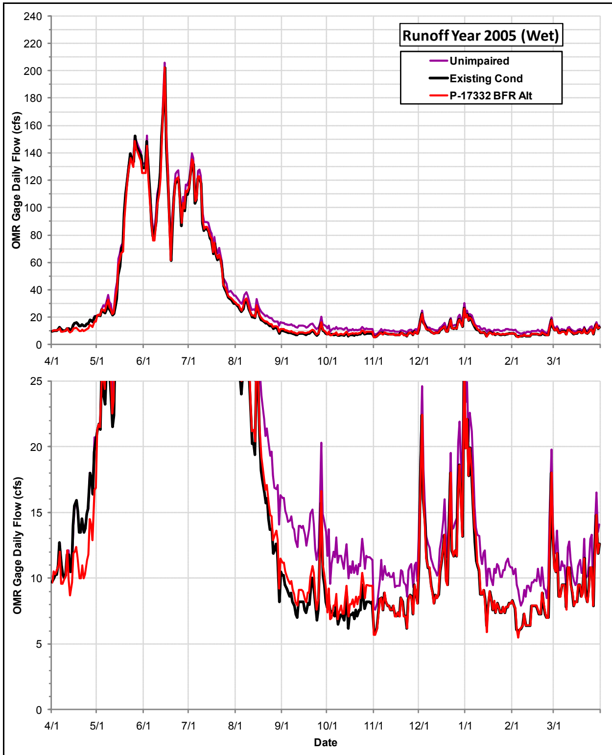
Daily Flows (cfs) at the OMR Gage under the Permit 17332 Bypass Flow Requirements Alternative, the Existing Condition and the Index of Unimpaired Conditions during Runoff Year 2005
