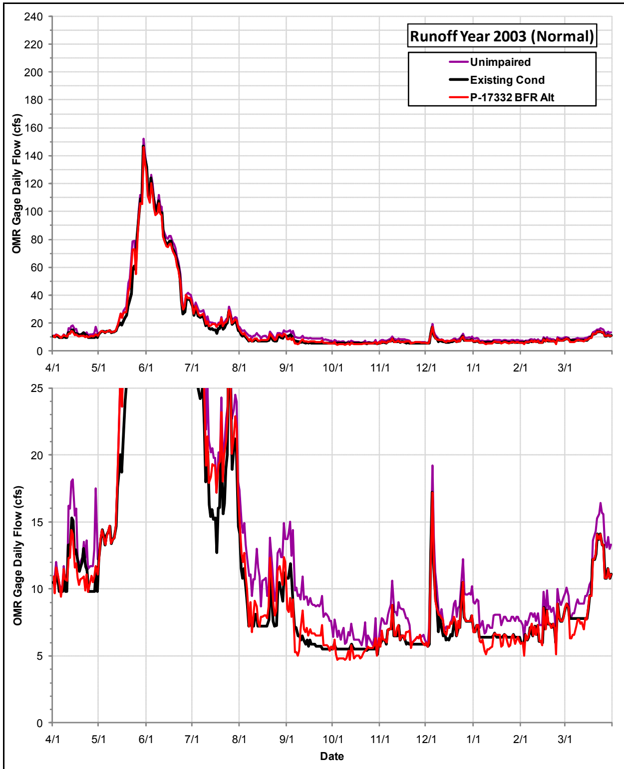
Daily Flows (cfs) at the OMR Gage under the Permit 17332 Bypass Flow Requirements Alternative, the Existing Condition and the Index of Unimpaired Conditions during Runoff Year 2003
