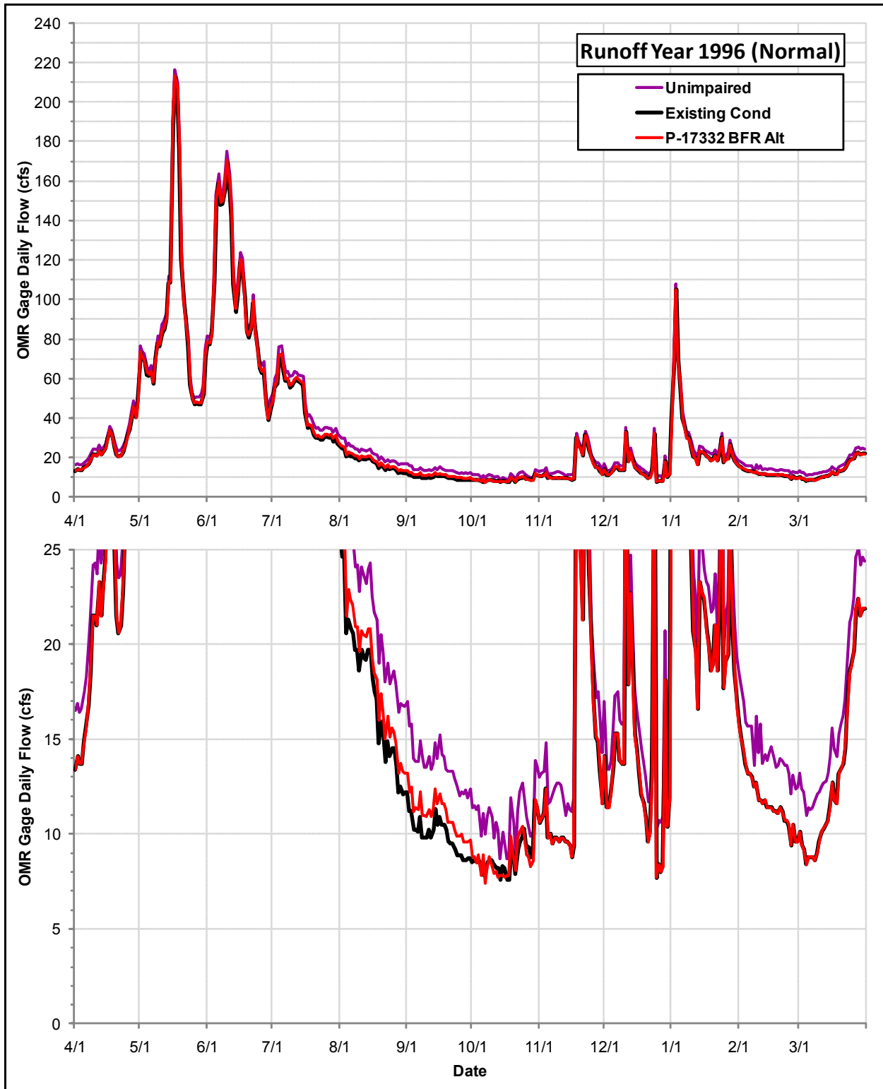
Daily Flows (cfs) at the OMR Gage under the Permit 17332 Bypass Flow Requirements Alternative, the Existing Condition and the Index of Unimpaired Conditions during Runoff Year 1996
