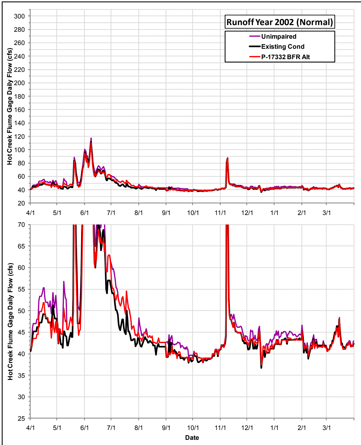
Daily Flows (cfs) at the USGS Hot Creek Flume Gage under the Permit 17332 Bypass Flow Requirements Alternative, the Existing Condition and the Index of Unimpaired Conditions during Runoff Year 2002
