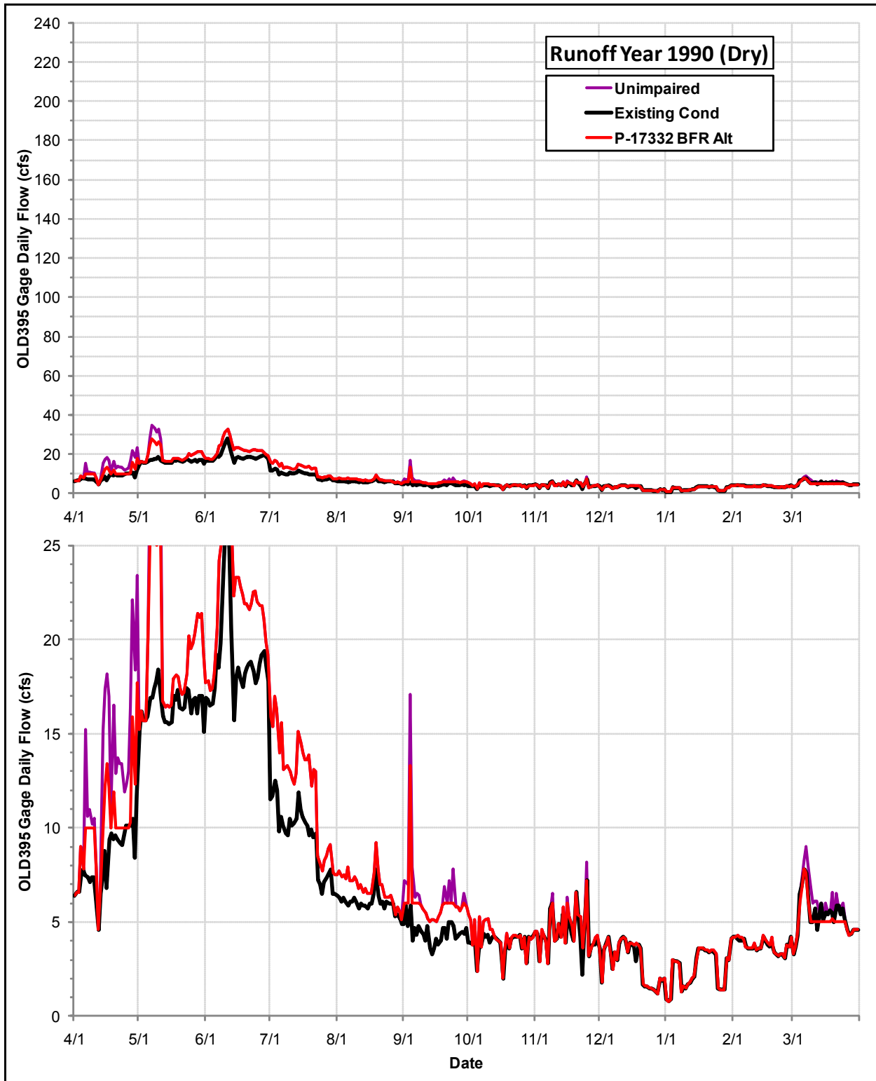
Daily Flows (cfs) at the OLD395 Gage under the Permit 17332 Bypass Flow Requirements Alternative, the Existing Condition and the Index of Unimpaired Conditions during Runoff Year 1990
