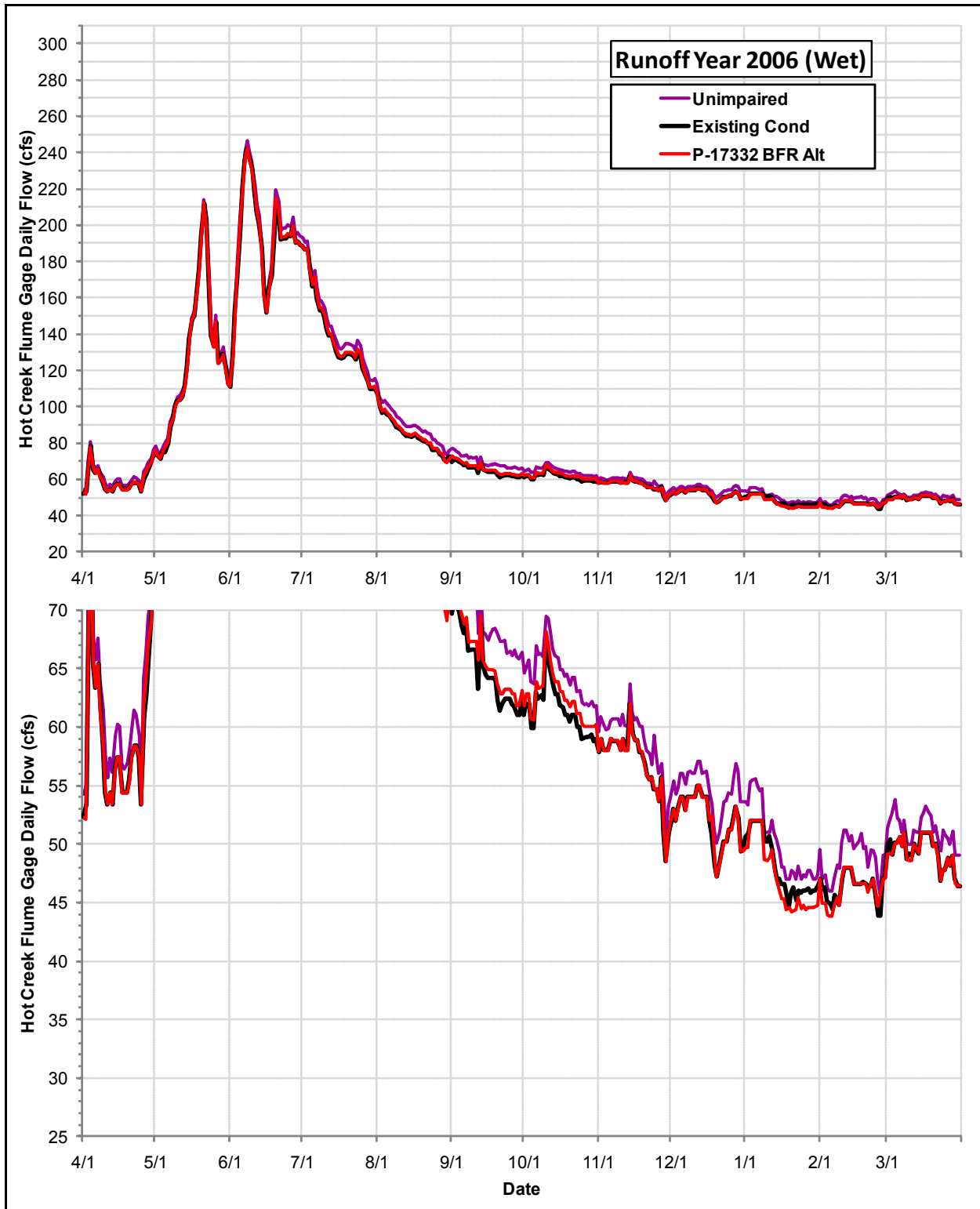
Daily Flows (cfs) at the USGS Hot Creek Flume Gage under the Permit 17332 Bypass Flow Requirements Alternative, the Existing Condition and the Index of Unimpaired Conditions during Runoff Year 2006
