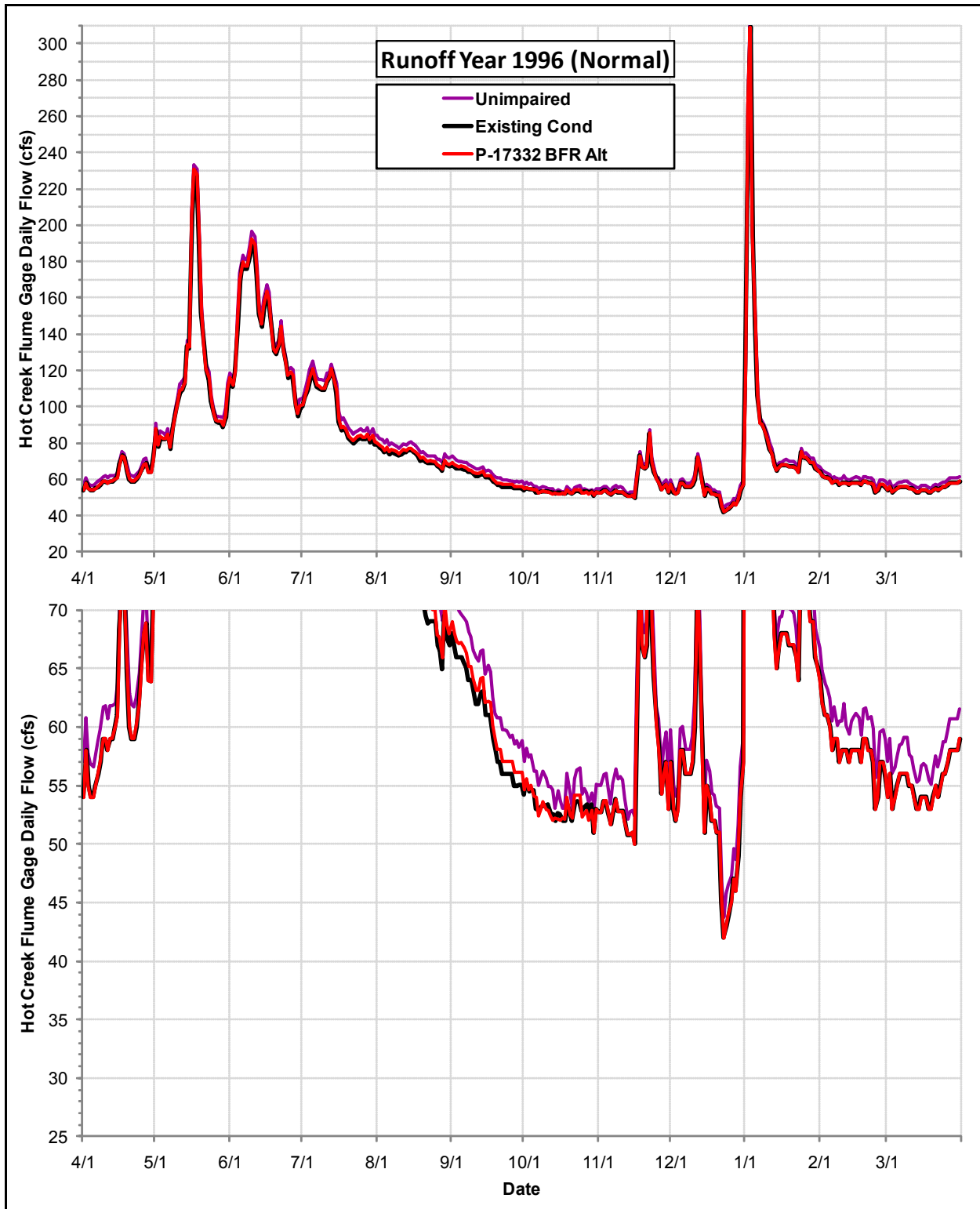
Daily Flows (cfs) at the USGS Hot Creek Flume Gage under the Permit 17332 Bypass Flow Requirements Alternative, the Existing Condition and the Index of Unimpaired Conditions during Runoff Year 1996
