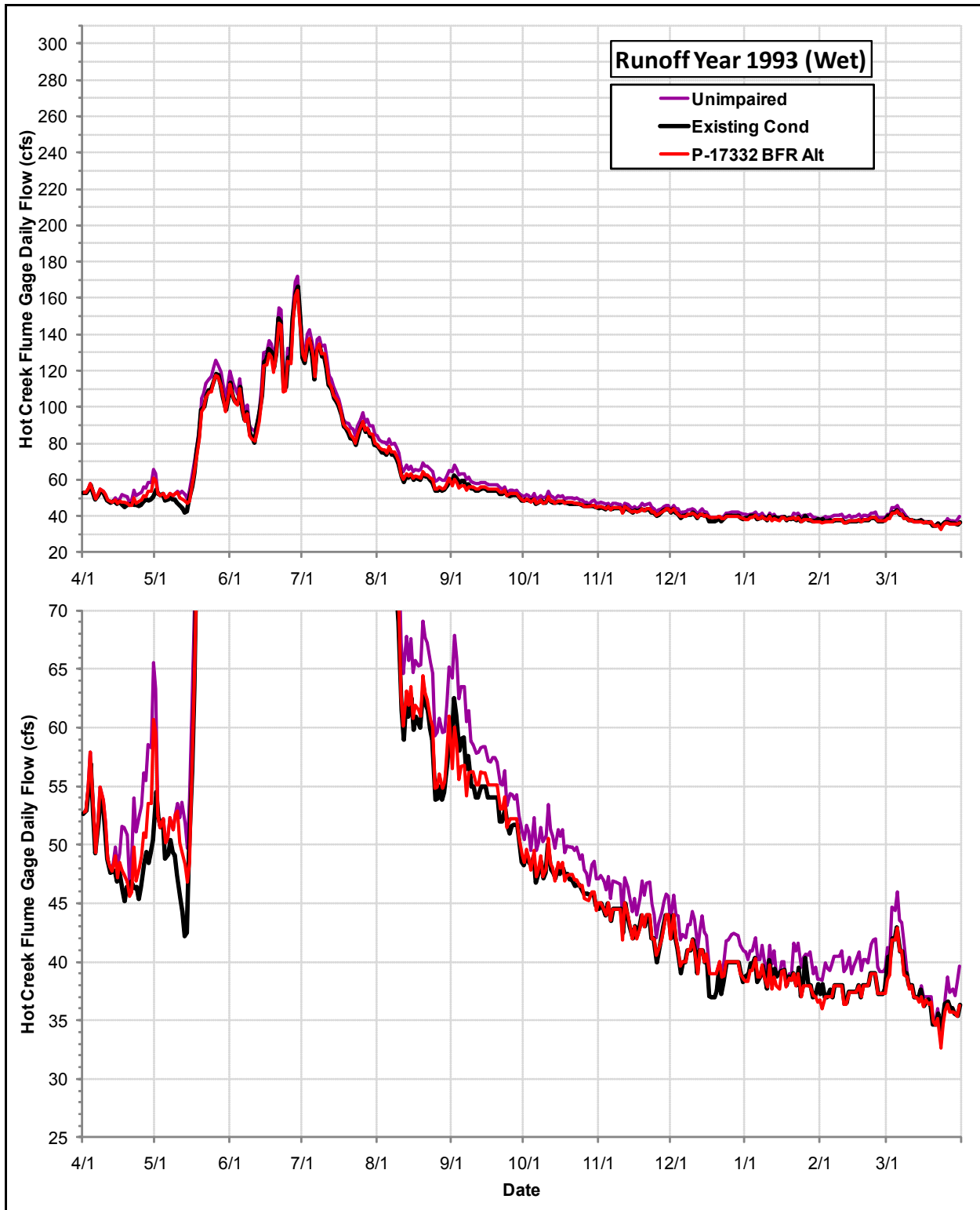
Daily Flows (cfs) at the USGS Hot Creek Flume Gage under the Permit 17332 Bypass Flow Requirements Alternative, the Existing Condition and the Index of Unimpaired Conditions during Runoff Year 1993
