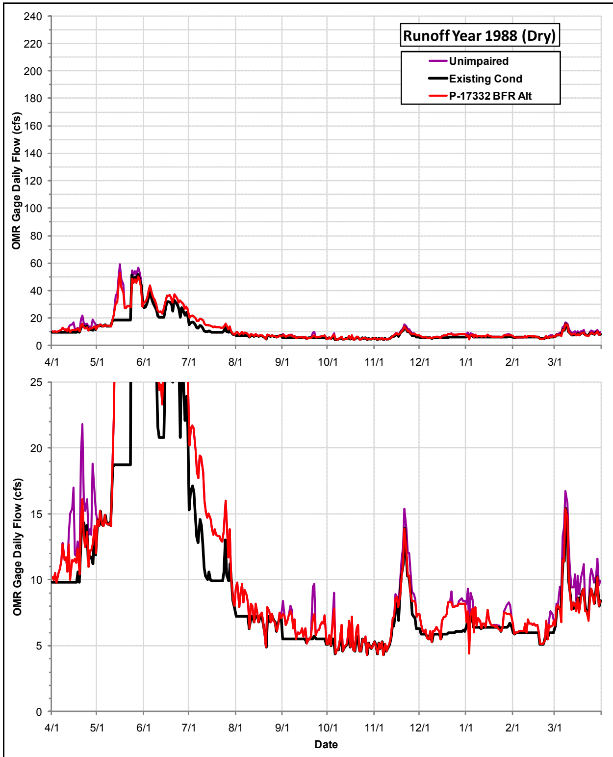
Daily Flows (cfs) at the OMR Gage under the Permit 17332 Bypass Flow Requirements Alternative, the Existing Condition and the Index of Unimpaired Conditions during Runoff Year 1988
