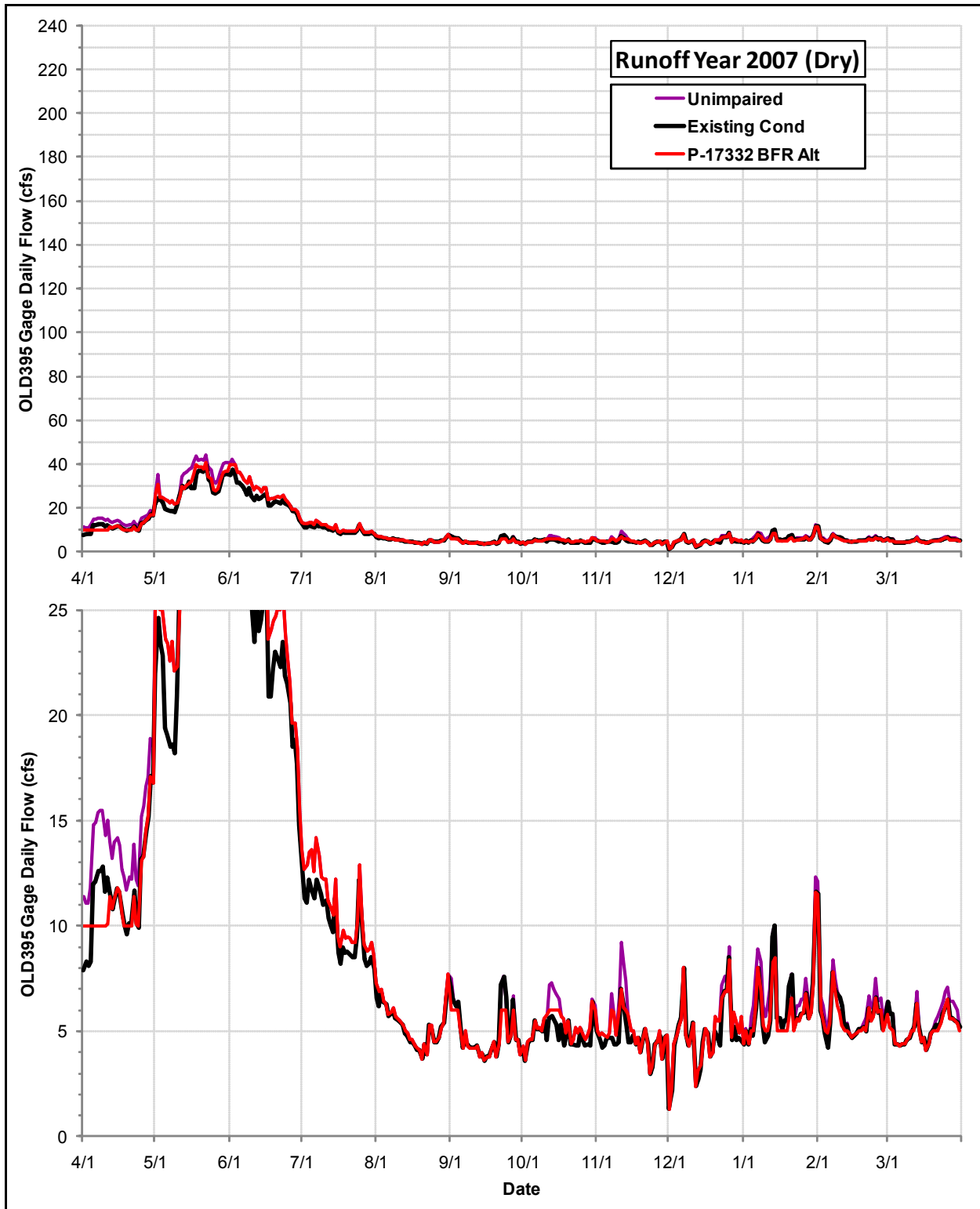
Daily Flows (cfs) at the OLD395 Gage under the Permit 17332 Bypass Flow Requirements Alternative, the Existing Condition and the Index of Unimpaired Conditions during Runoff Year 2007
