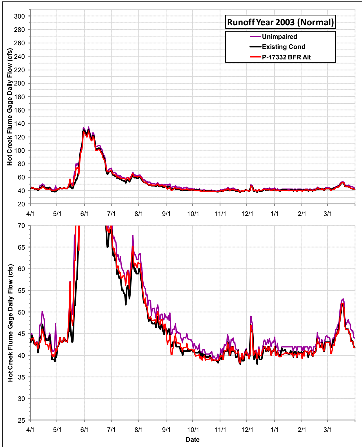
Daily Flows (cfs) at the USGS Hot Creek Flume Gage under the Permit 17332 Bypass Flow Requirements Alternative, the Existing Condition and the Index of Unimpaired Conditions during Runoff Year 2003
