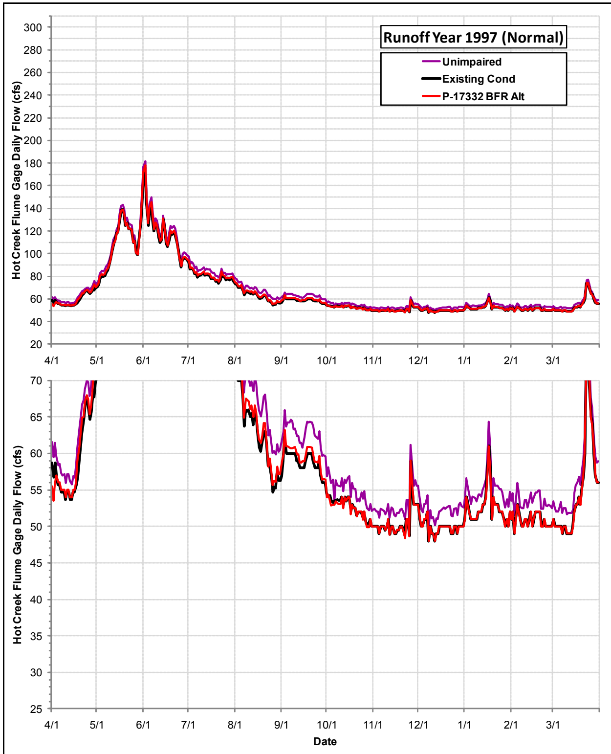
Daily Flows (cfs) at the USGS Hot Creek Flume Gage under the Permit 17332 Bypass Flow Requirements Alternative, the Existing Condition and the Index of Unimpaired Conditions during Runoff Year 1997
