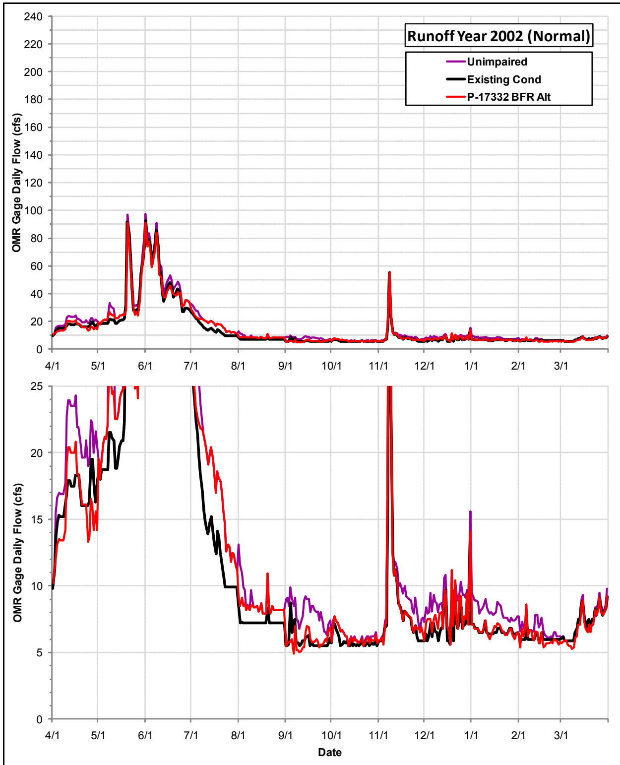
Daily Flows (cfs) at the OMR Gage under the Permit 17332 Bypass Flow Requirements Alternative, the Existing Condition and the Index of Unimpaired Conditions during Runoff Year 2002
