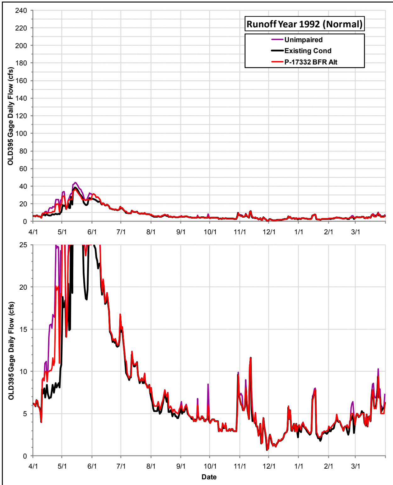
Daily Flows (cfs) at the OLD395 Gage under the Permit 17332 Bypass Flow Requirements Alternative, the Existing Condition and the Index Unimpaired Conditions during Runoff Year 1992
