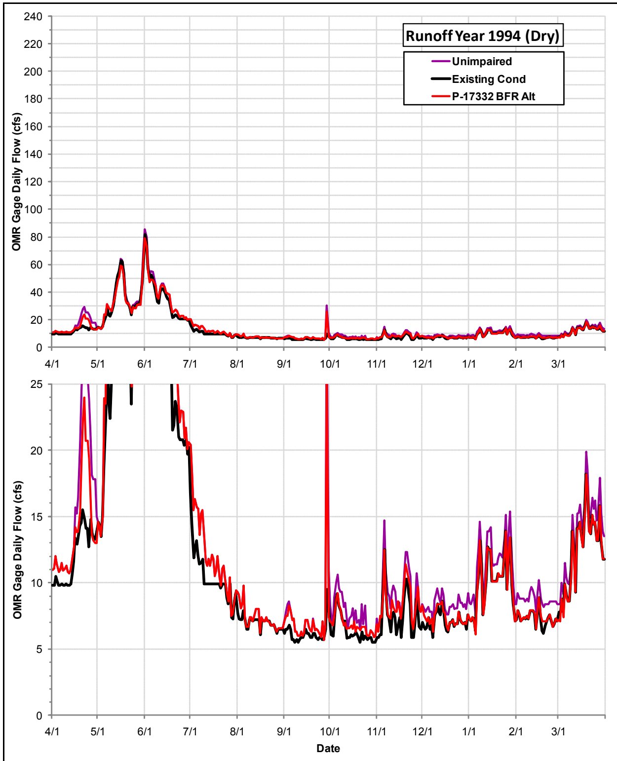
Daily Flows (cfs) at the OMR Gage under the Permit 17332 Bypass Flow Requirements Alternative, the Existing Condition and the Index of Unimpaired Conditions during Runoff Year 1994
