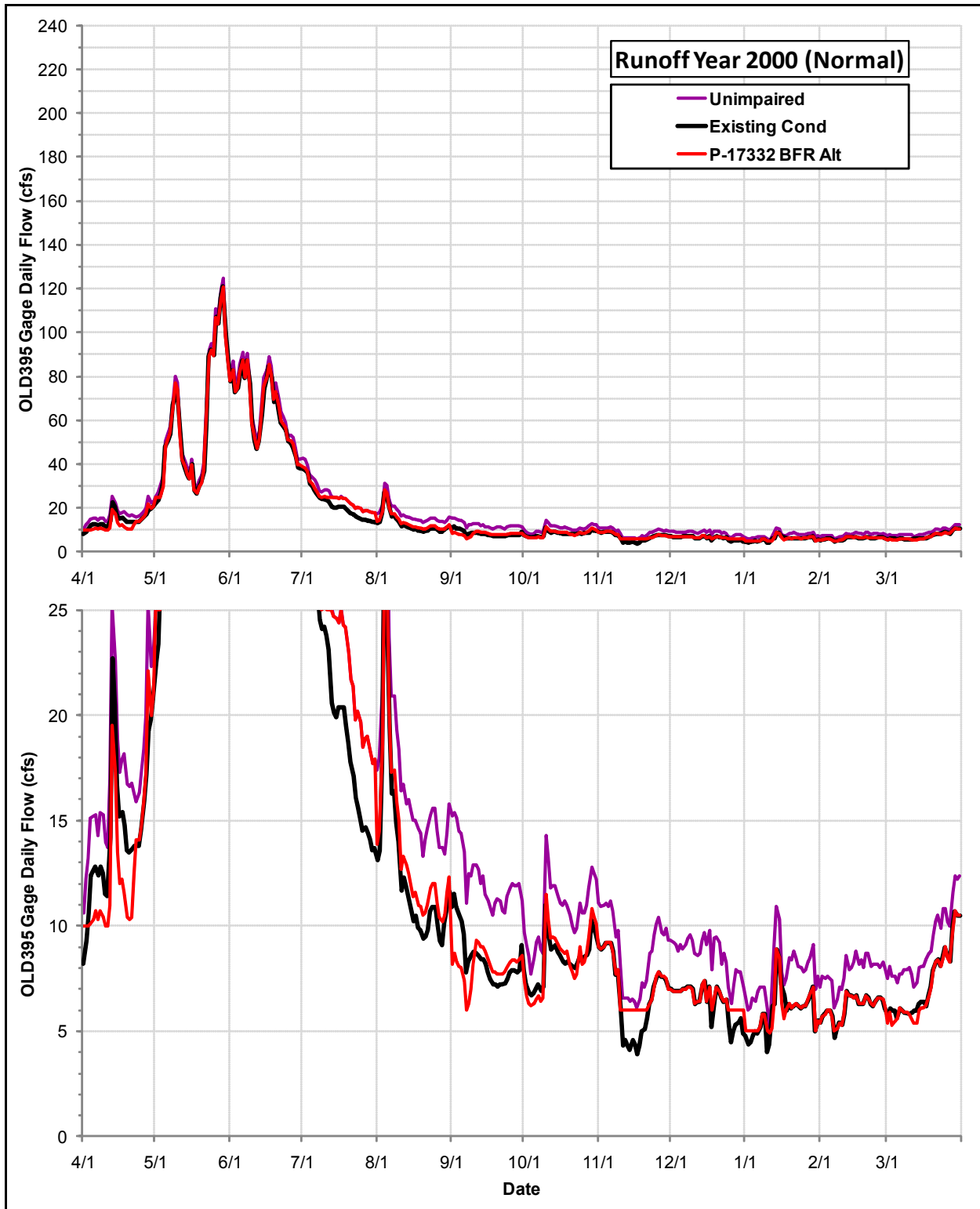
Daily Flows (cfs) at the OLD395 Gage under the Permit 17332 Bypass Flow Requirements Alternative, the Existing Condition and the Index of Unimpaired Conditions during Runoff Year 2000
