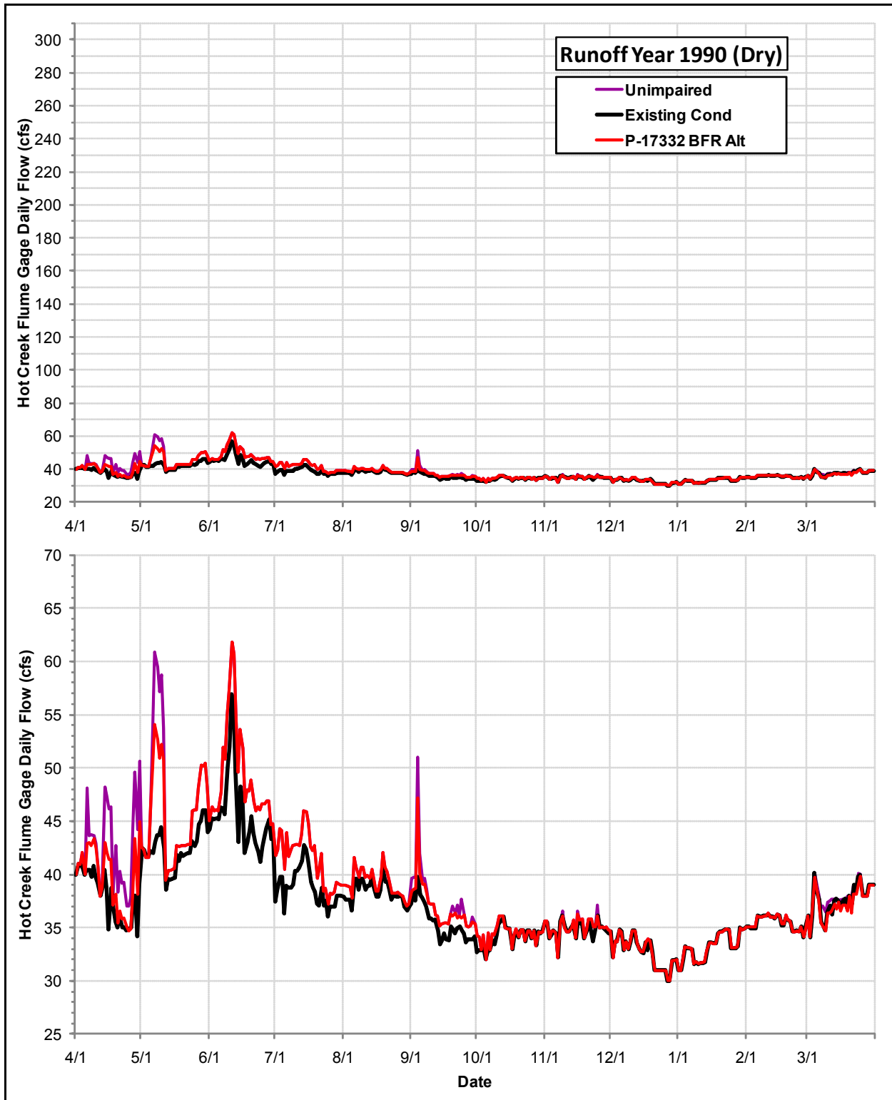
Daily Flows (cfs) at the USGS Hot Creek Flume Gage under the Permit 17332 Bypass Flow Requirements Alternative, the Existing Condition and the Index of Unimpaired Conditions during Runoff Year 1990
