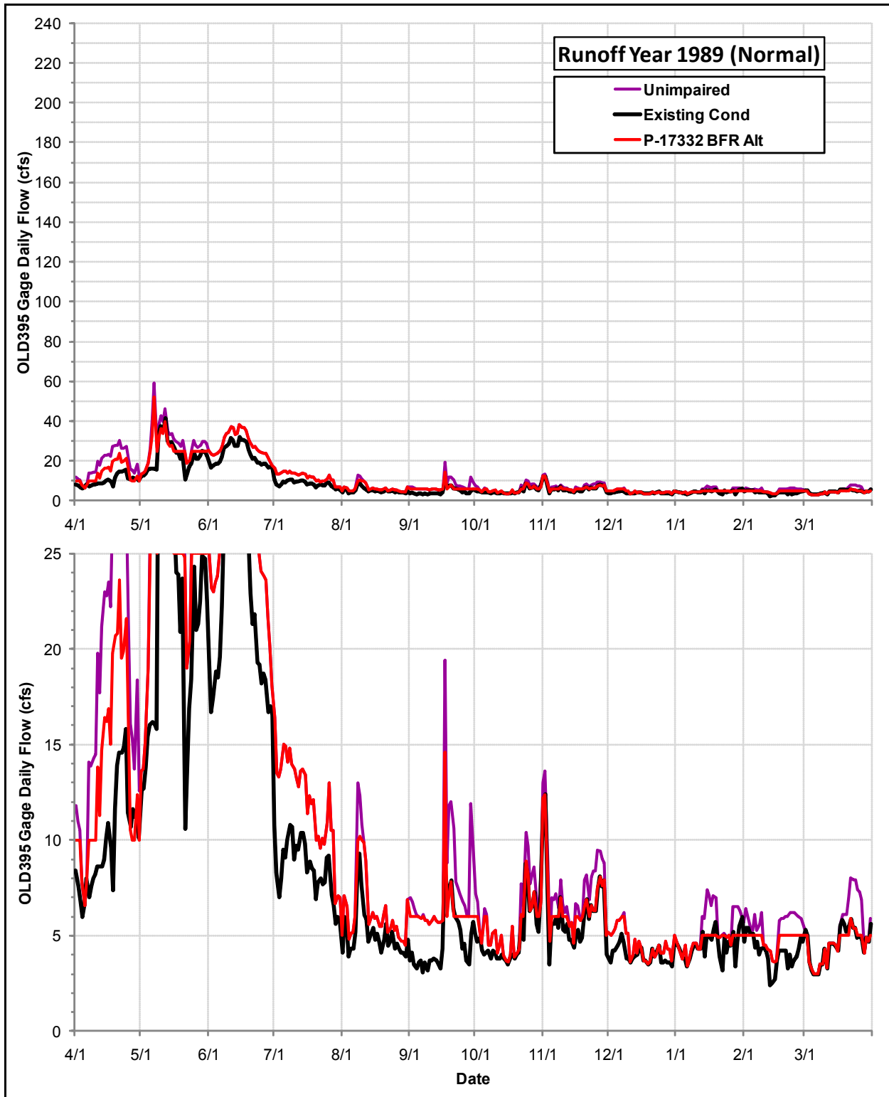
Daily Flows (cfs) at the OLD395 Gage under the Permit 17332 Bypass Flow Requirements Alternative, the Existing Condition and the Index of Unimpaired Conditions during Runoff Year 1989
