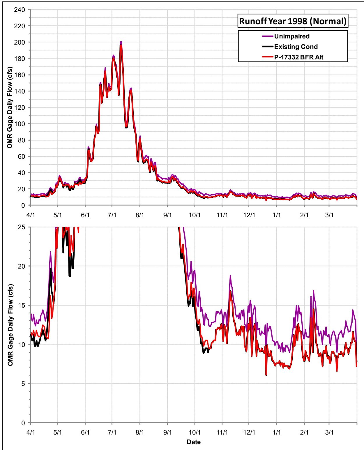
Daily Flows (cfs) at the OMR Gage under the Permit 17332 Bypass Flow Requirements Alternative, the Existing Condition and the Index of Unimpaired Conditions during Runoff Year 1998
