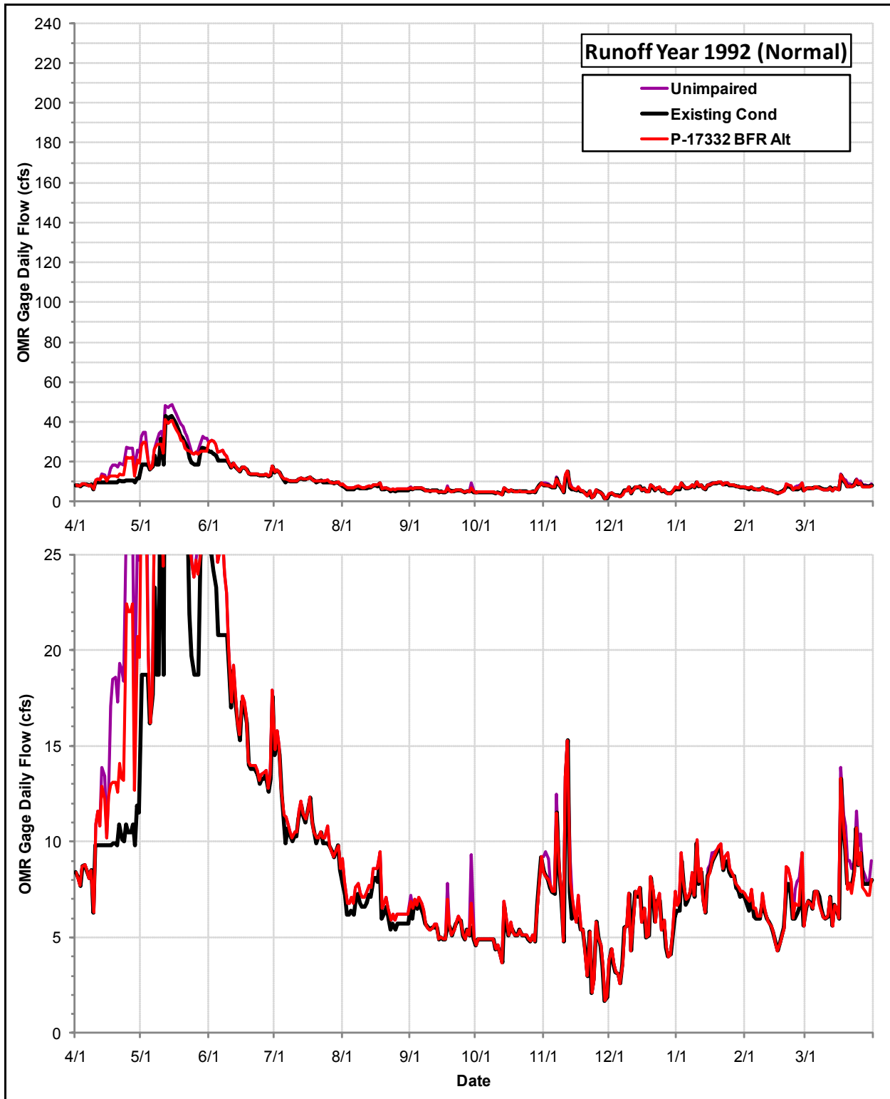
Daily Flows (cfs) at the OMR Gage under the Permit 17332 Bypass Flow Requirements Alternative, the Existing Condition and the Index Unimpaired Conditions during Runoff Year 1992
