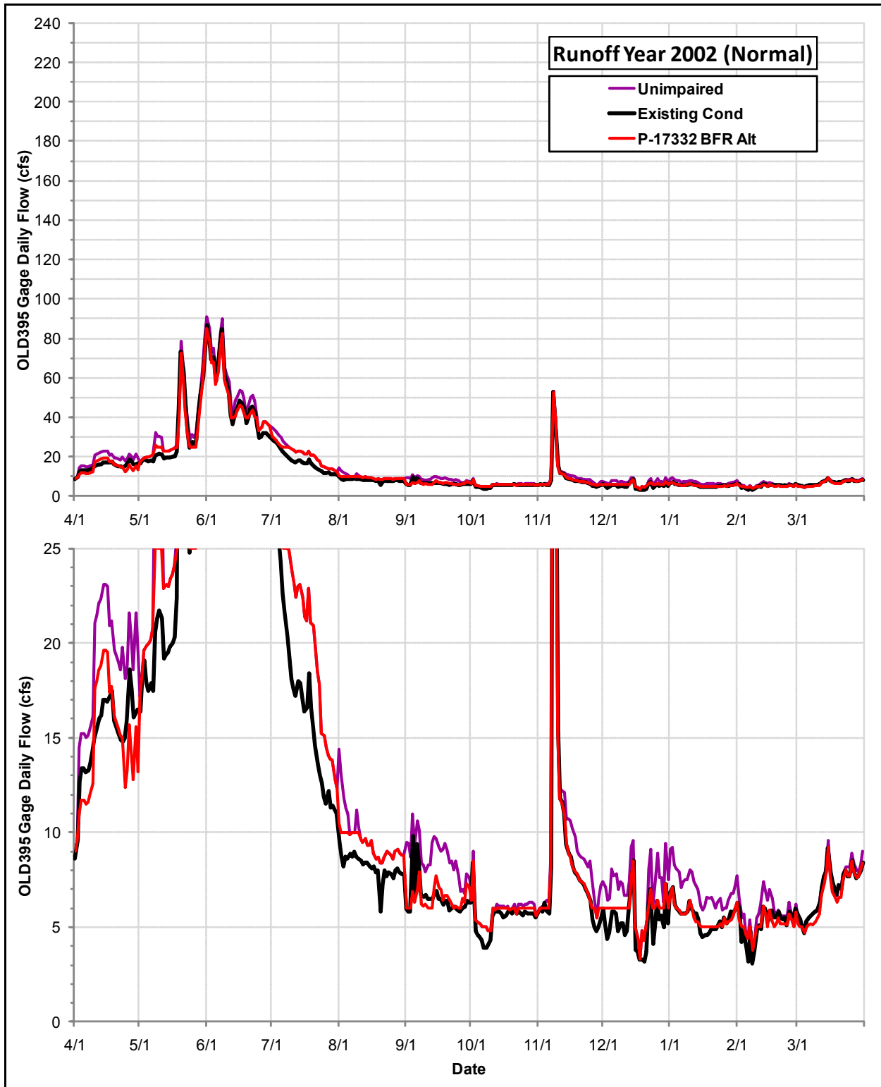
Daily Flows (cfs) at the OLD395 Gage under the Permit 17332 Bypass Flow Requirements Alternative, the Existing Condition and the Index of Unimpaired Conditions during Runoff Year 2002
