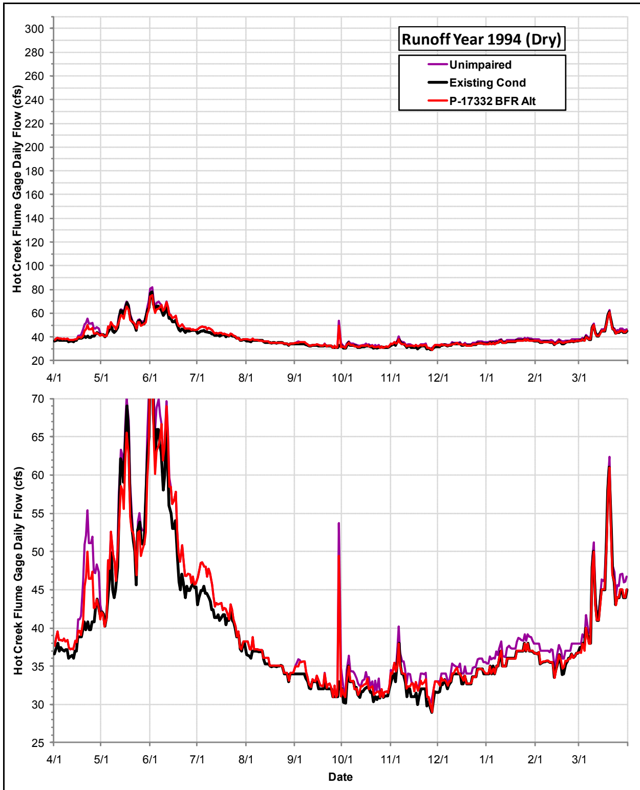
Daily Flows (cfs) at the USGS Hot Creek Flume Gage under the Permit 17332 Bypass Flow Requirements Alternative, the Existing Condition and the Index of Unimpaired Conditions during Runoff Year 1994
