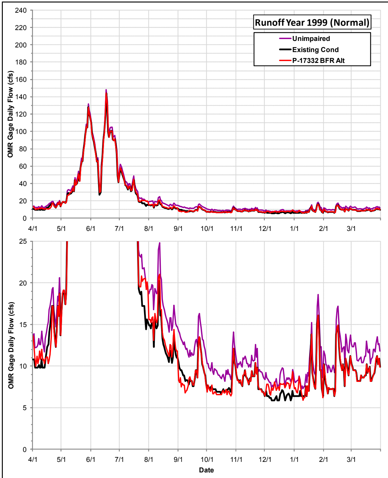
Daily Flows (cfs) at the OMR Gage under the Permit 17332 Bypass Flow Requirements Alternative, the Existing Condition and the Index of Unimpaired Conditions during Runoff Year 1999
