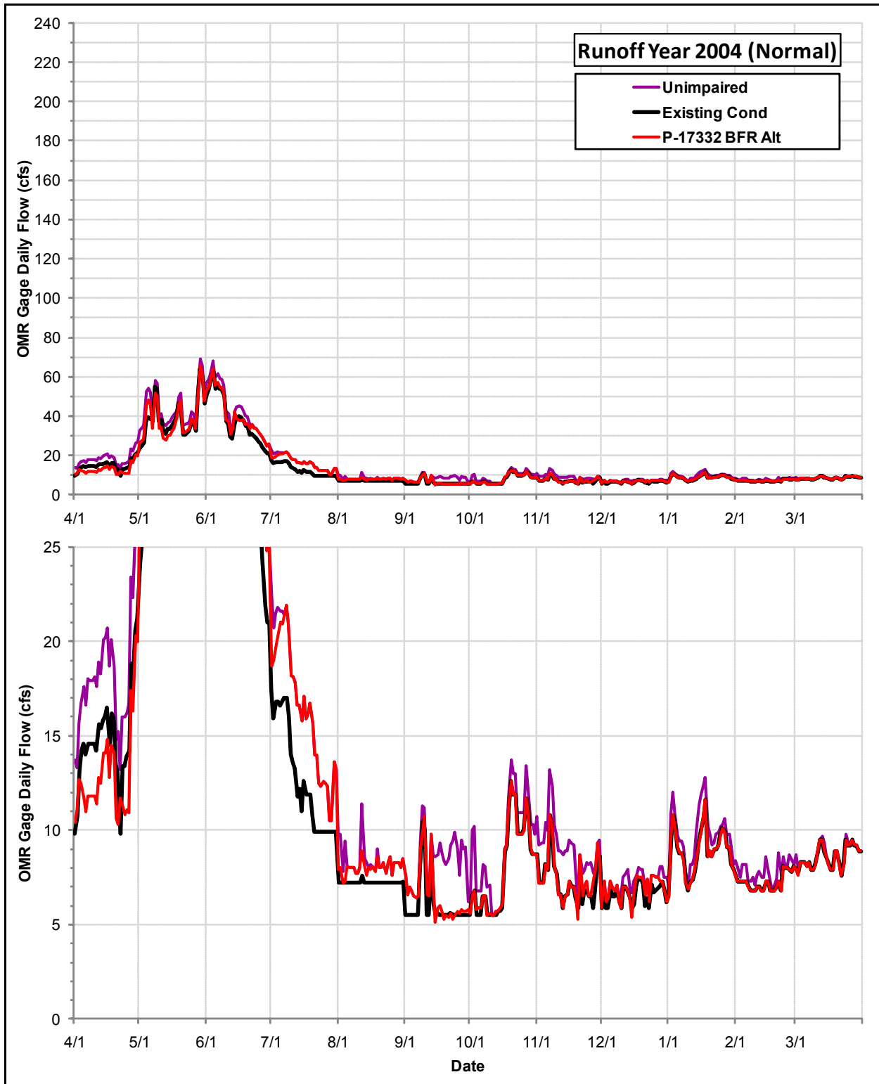
Daily Flows (cfs) at the OMR Gage under the Permit 17332 Bypass Flow Requirements Alternative, the Existing Condition and the Index of Unimpaired Conditions during Runoff Year 2004
