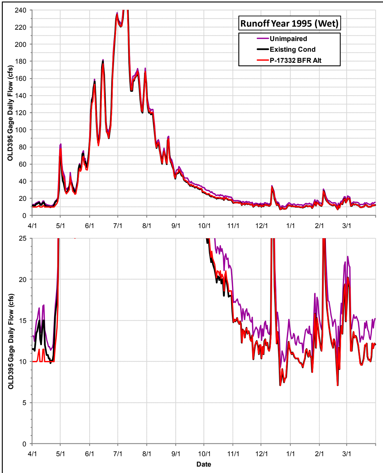
Daily Flows (cfs) at the OLD395 Gage under the Permit 17332 Bypass Flow Requirements Alternative, the Existing Condition and the Index of Unimpaired Conditions during Runoff Year 1995
