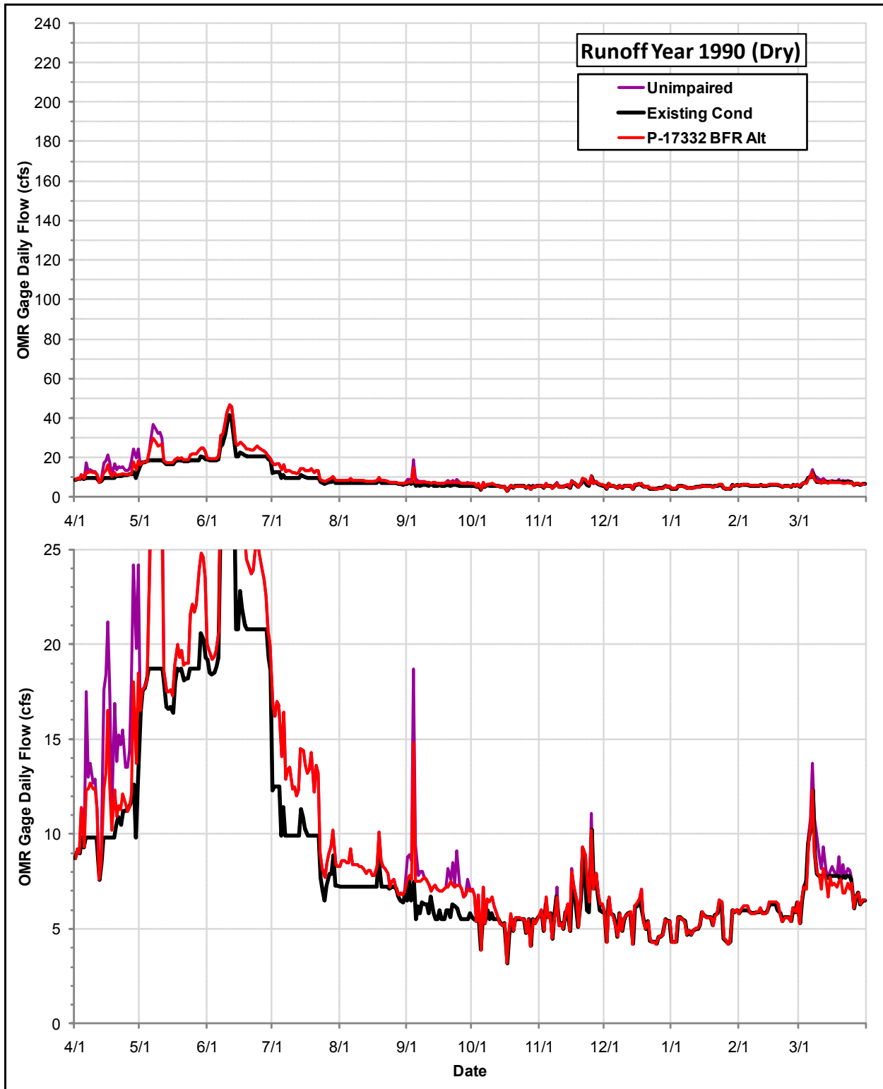
Daily Flows (cfs) at the OMR Gage under the Permit 17332 Bypass Flow Requirements Alternative, the Existing Condition and the Index of Unimpaired Conditions during Runoff Year 1990
