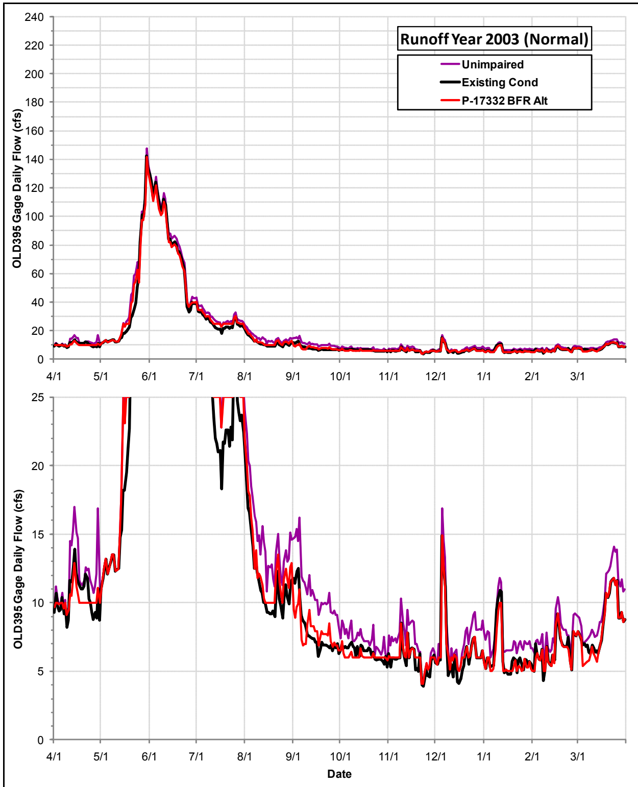
Daily Flows (cfs) at the OLD395 Gage under the Permit 17332 Bypass Flow Requirements Alternative, the Existing Condition and the Index of Unimpaired Conditions during Runoff Year 2003
