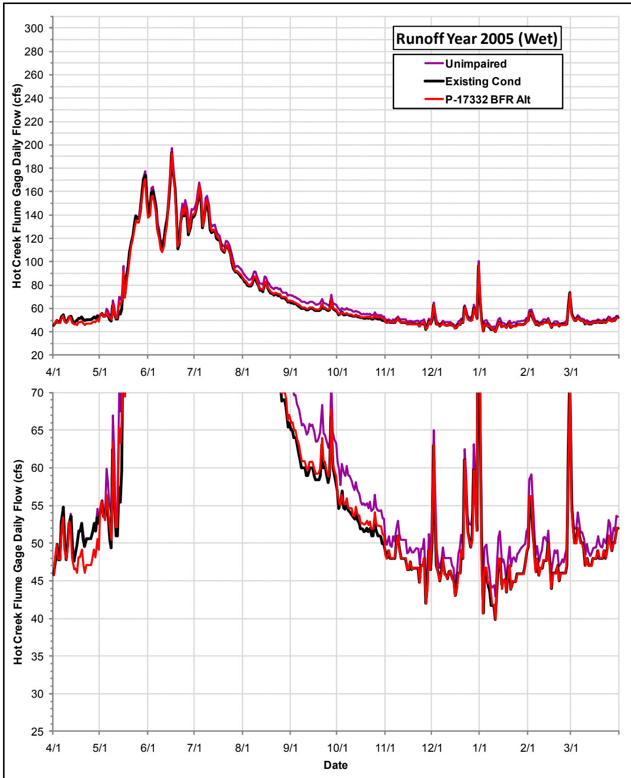
Daily Flows (cfs) at the USGS Hot Creek Flume Gage under the Permit 17332 Bypass Flow Requirements Alternative, the Existing Condition and the Index of Unimpaired Conditions during Runoff Year 2005
