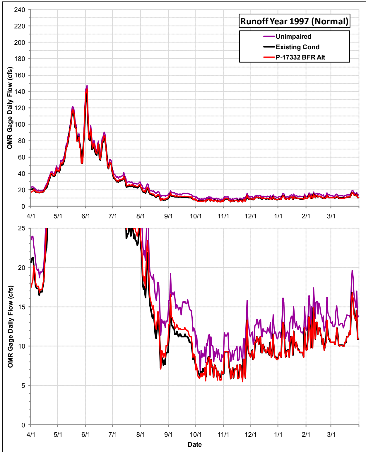
Daily Flows (cfs) at the OMR Gage under the Permit 17332 Bypass Flow Requirements Alternative, the Existing Condition and the Index of Unimpaired Conditions during Runoff Year 1997
