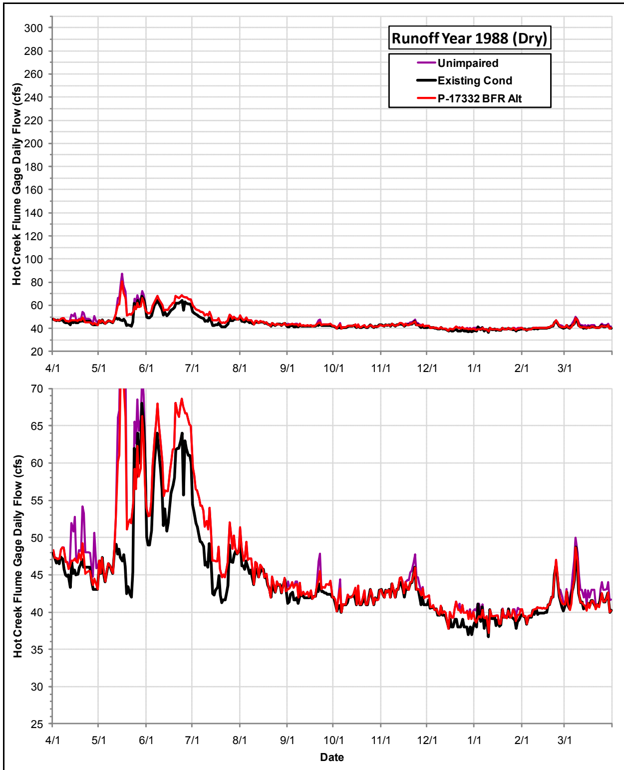
Daily Flows (cfs) at the USGS Hot Creek Flume Gage under the Permit 17332 Bypass Flow Requirements Alternative, the Existing Condition and the Index of Unimpaired Conditions during Runoff Year 1988
