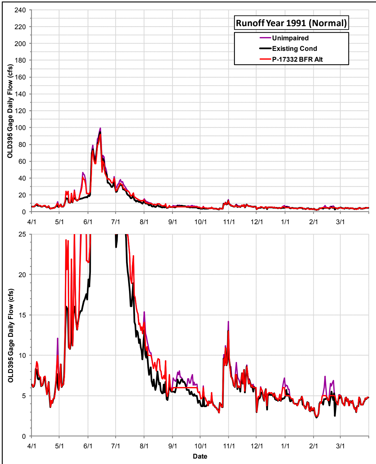
Daily Flows (cfs) at the OLD395 Gage under the Permit 17332 Bypass Flow Requirements Alternative, the Existing Condition and the Index of Unimpaired Conditions during Runoff Year 1991
