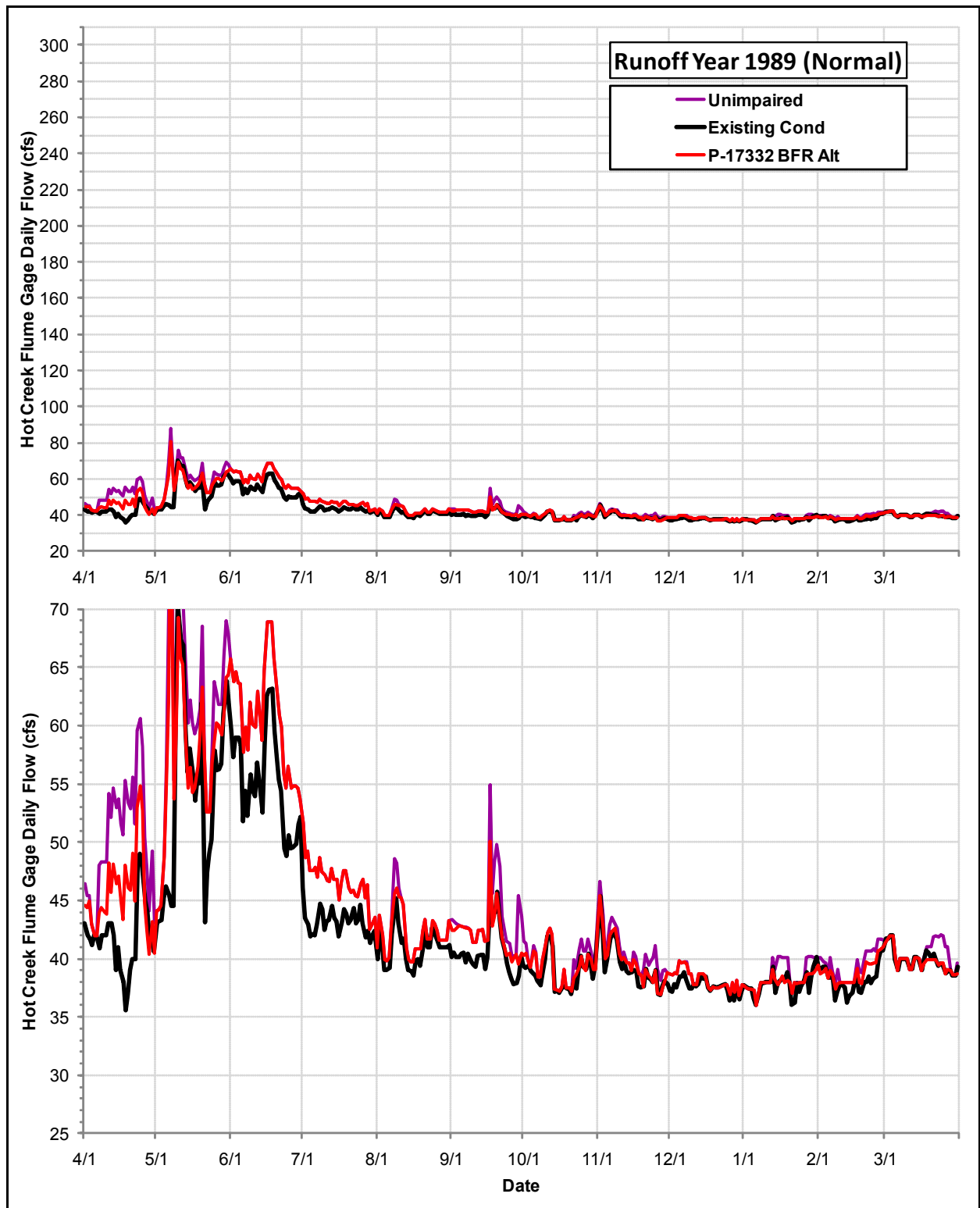
Daily Flows (cfs) at the USGS Hot Creek Flume Gage under the Permit 17332 Bypass Flow Requirements Alternative, the Existing Condition and the Index of Unimpaired Conditions during Runoff Year 1989
