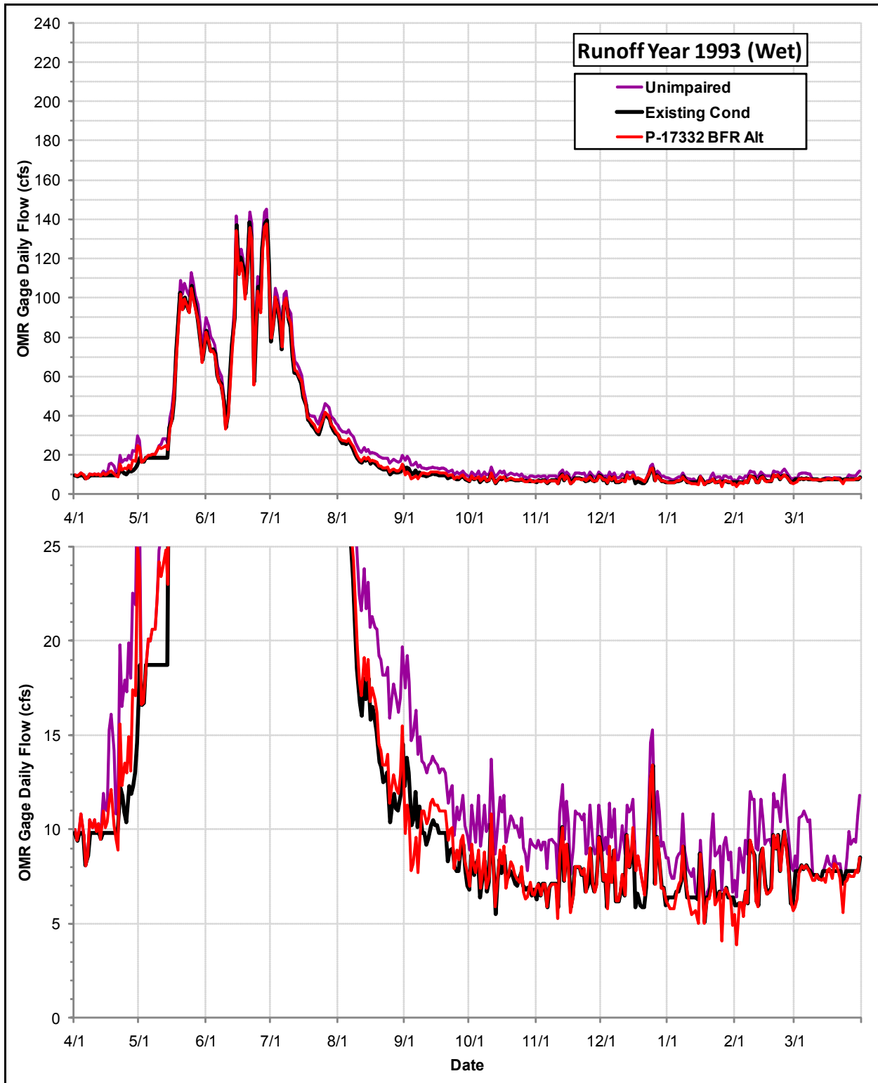
Daily Flows (cfs) at the OMR Gage under the Permit 17332 Bypass Flow Requirements Alternative, the Existing Condition and the Index of Unimpaired Conditions during Runoff Year 1993
