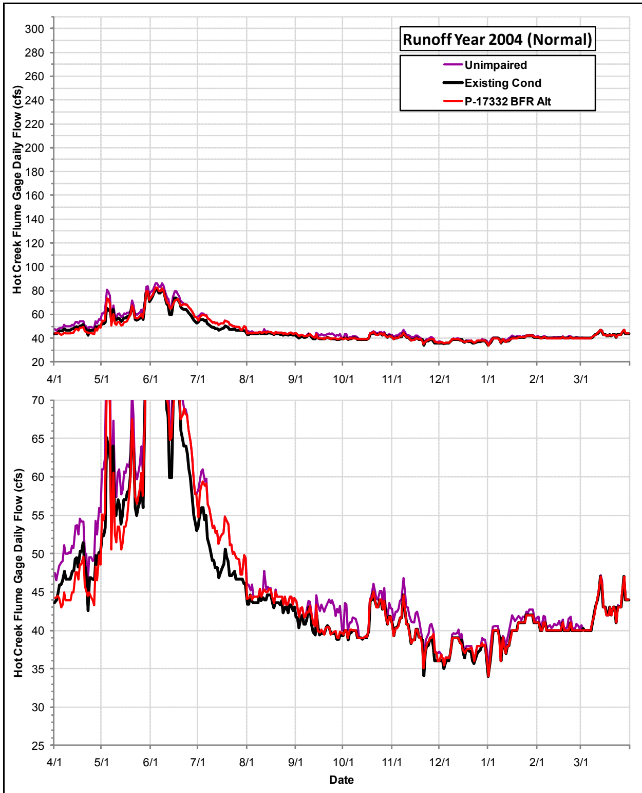
Daily Flows (cfs) at the USGS Hot Creek Flume Gage under the Permit 17332 Bypass Flow Requirements Alternative, the Existing Condition and the Index of Unimpaired Conditions during Runoff Year 2004
