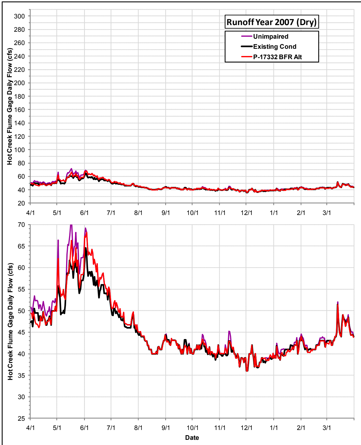
Daily Flows (cfs) at the USGS Hot Creek Flume Gage under the Permit 17332 Bypass Flow Requirements Alternative, the Existing Condition and the Index of Unimpaired Conditions during Runoff Year 2007
