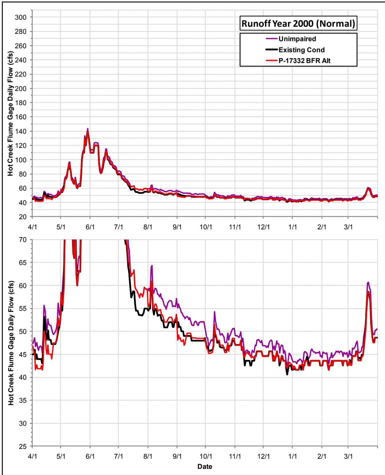
Daily Flows (cfs) at the USGS Hot Creek Flume Gage under the Permit 17332 Bypass Flow Requirements Alternative, the Existing Condition and the Index of Unimpaired Conditions during Runoff Year 2000
