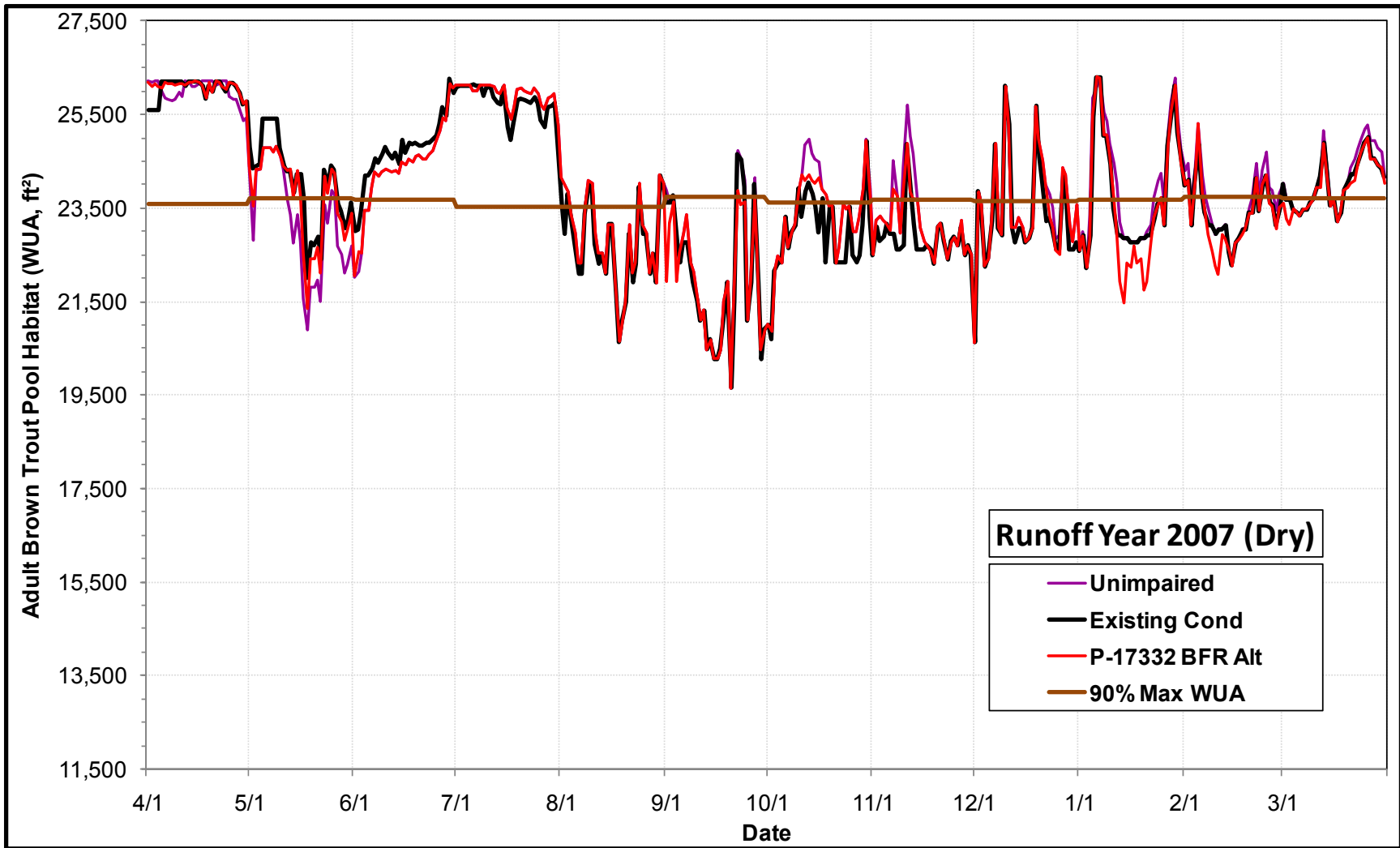
Daily Time Series Comparing Adult Brown Trout Pool Habitat Availability (WUA, ft 2 ) to 90% of Maximum (Theoretical) Habitat Availability under the Permit 17332 Bypass Flow Requirements Alternative, the Existing Condition and the Index of Unimpaired Conditions during Runoff Year 2007
