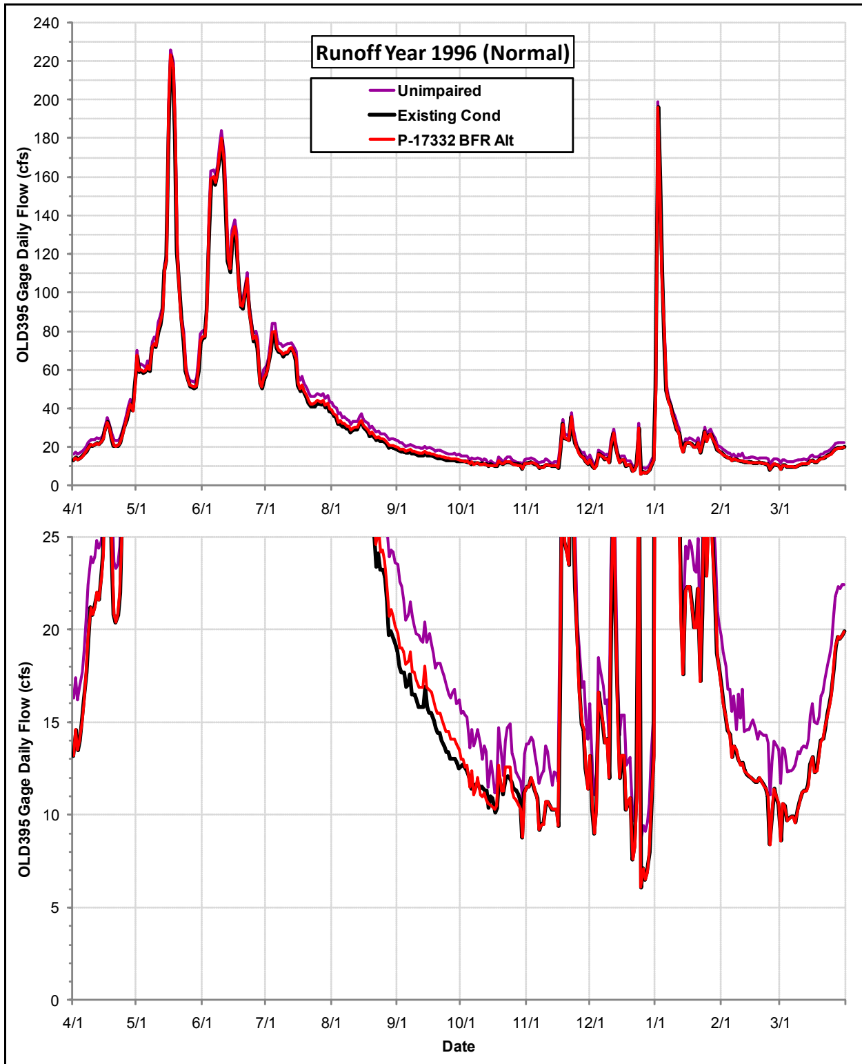
Daily Flows (cfs) at the OLD395 Gage under the Permit 17332 Bypass Flow Requirements Alternative, the Existing Condition and the Index of Unimpaired Conditions during Runoff Year 1996
