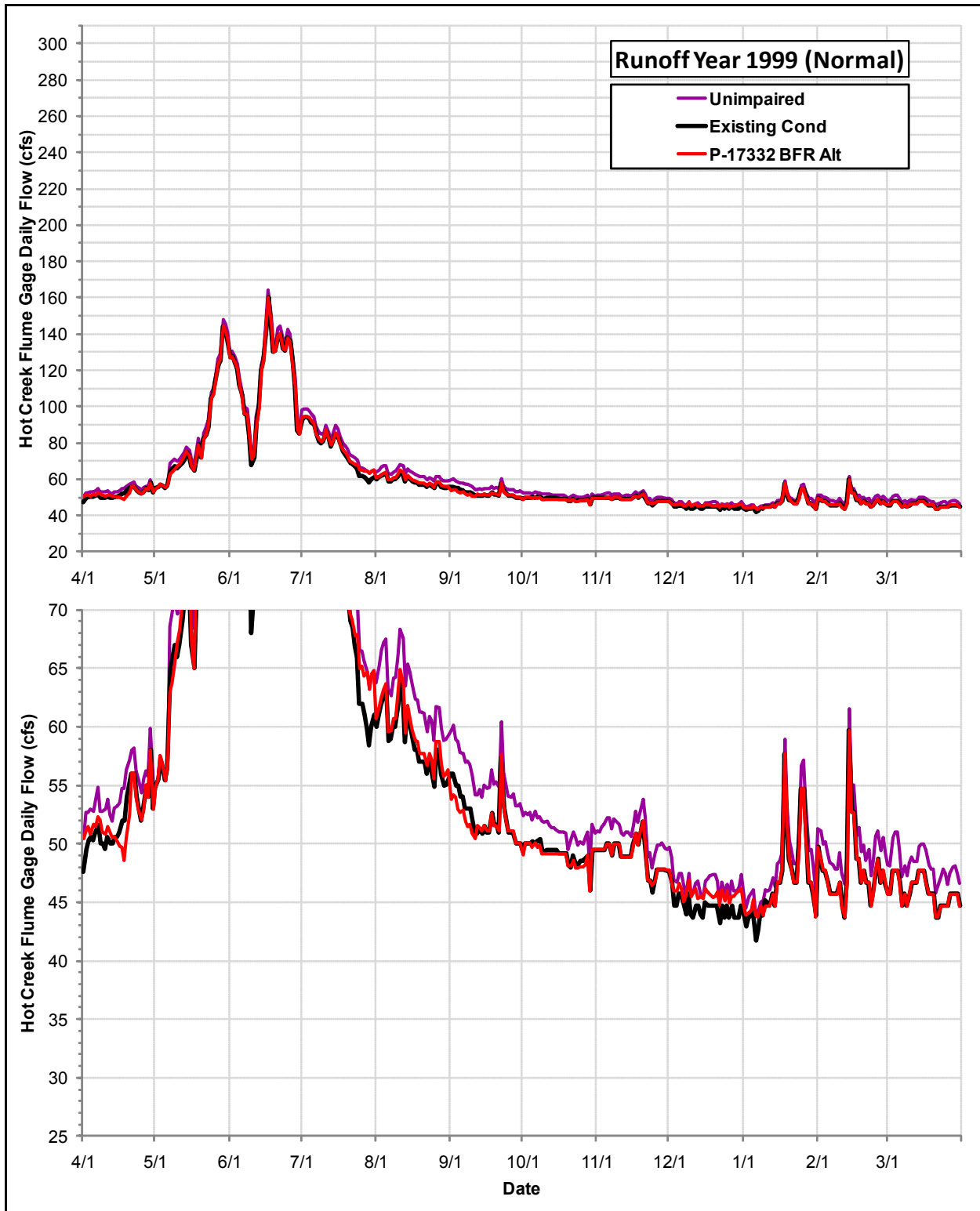
Daily Flows (cfs) at the USGS Hot Creek Flume Gage under the Permit 17332 Bypass Flow Requirements Alternative, the Existing Condition and the Index of Unimpaired Conditions during Runoff Year 1999
