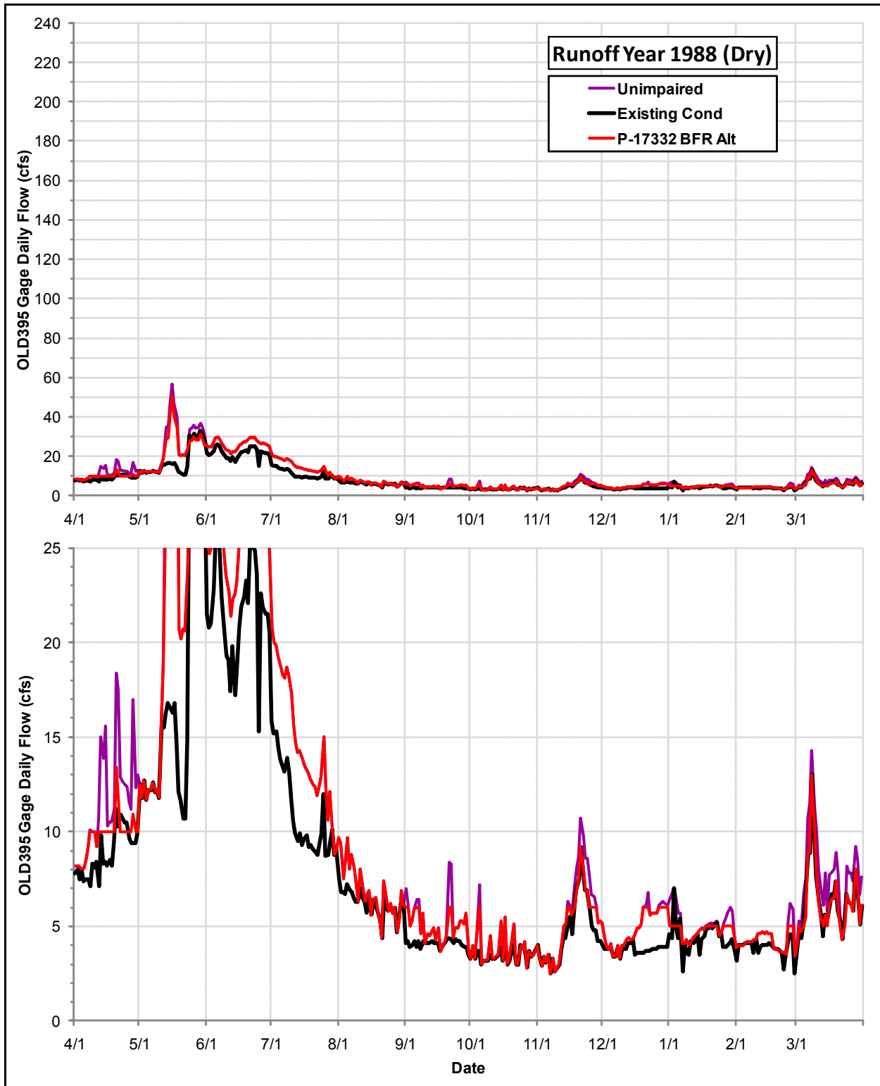
Daily Flows (cfs) at the OLD395 Gage under the Permit 17332 Bypass Flow Requirements Alternative, the Existing Condition and the Index of Unimpaired Conditions during Runoff Year 1988
