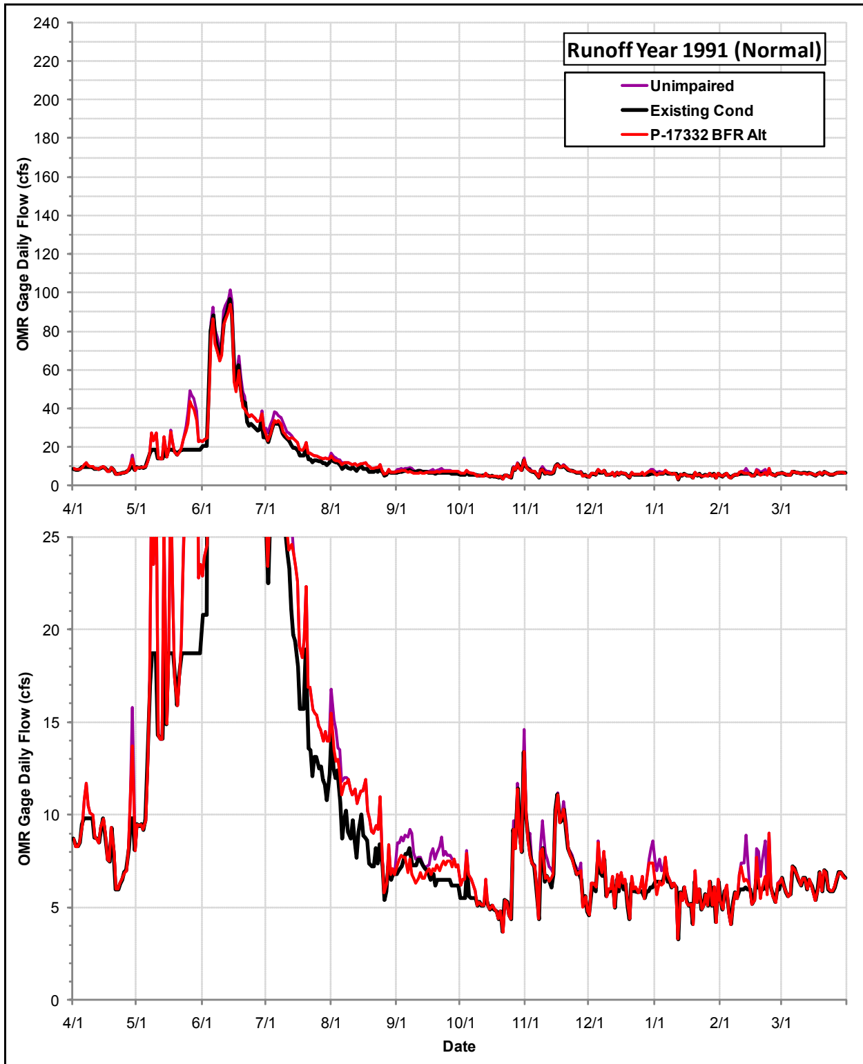
Daily Flows (cfs) at the OMR Gage under the Permit 17332 Bypass Flow Requirements Alternative, the Existing Condition and the Index of Unimpaired Conditions during Runoff Year 1991
