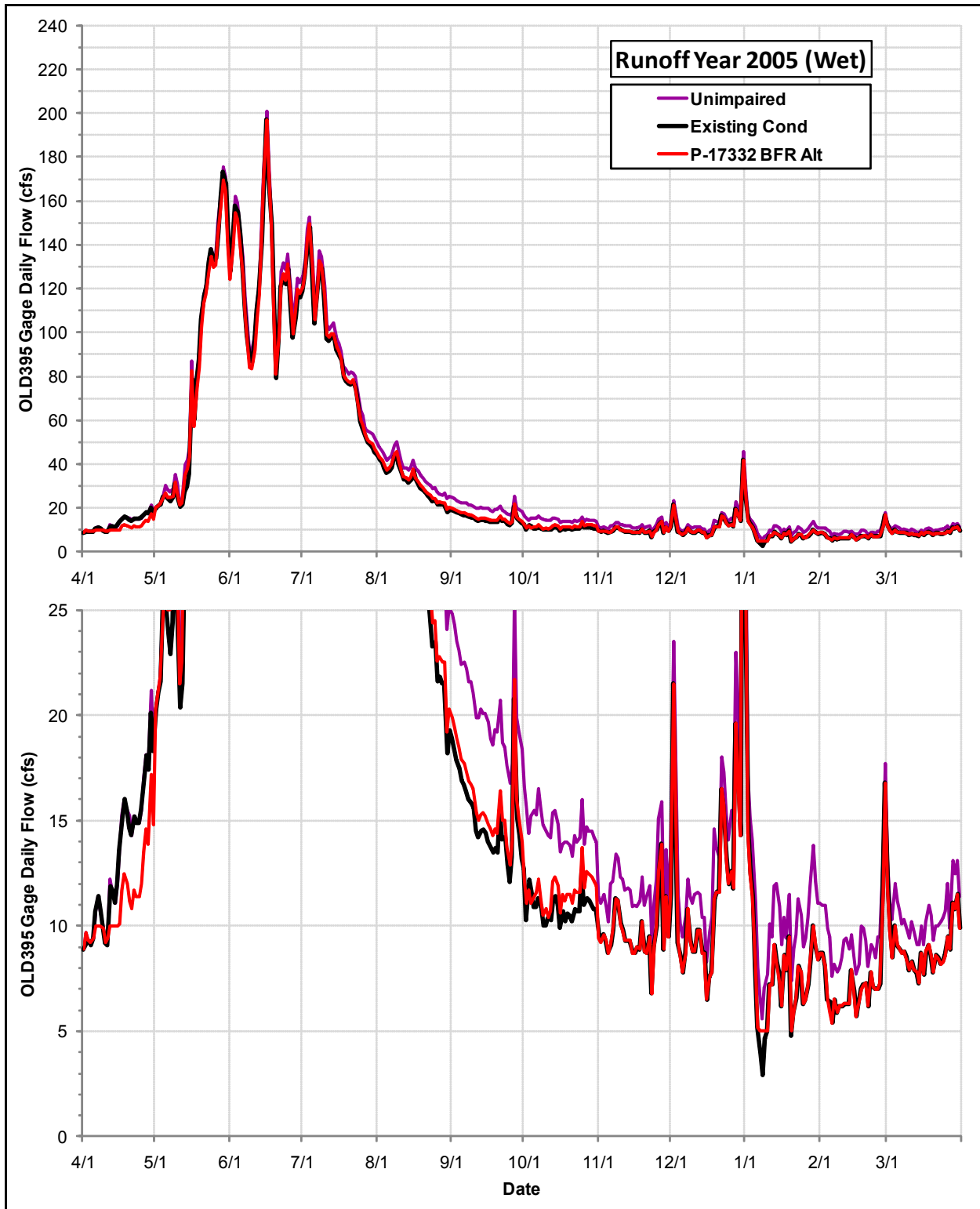
Daily Flows (cfs) at the OLD395 Gage under the Permit 17332 Bypass Flow Requirements Alternative, the Existing Condition and the Index of Unimpaired Conditions during Runoff Year 2005
