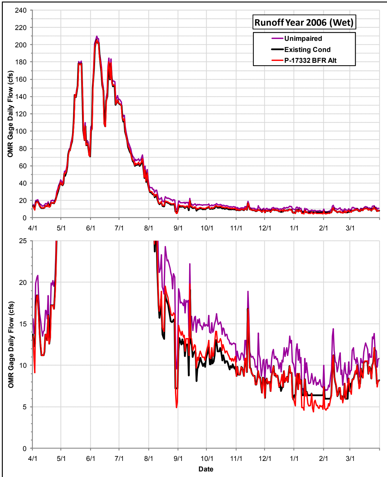
Daily Flows (cfs) at the OMR Gage under the Permit 17332 Bypass Flow Requirements Alternative, the Existing Condition and the Index of Unimpaired Conditions during Runoff Year 2006
