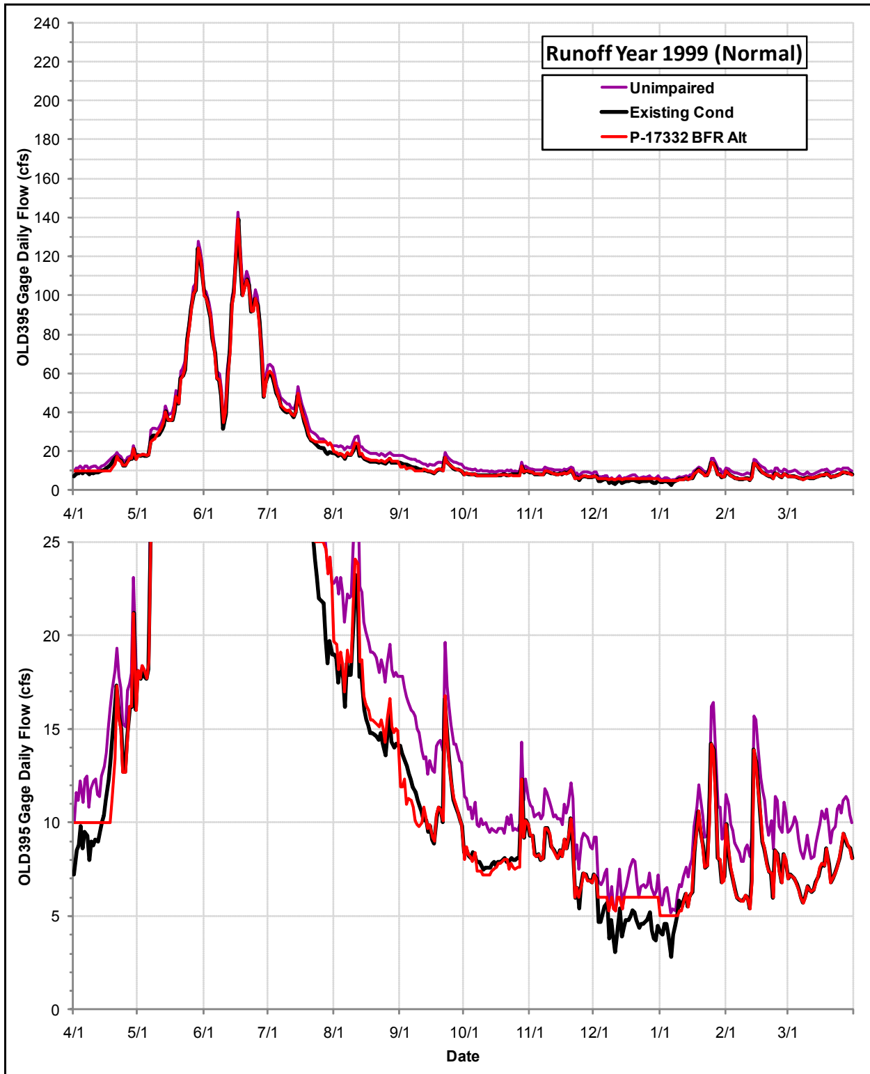
Daily Flows (cfs) at the OLD395 Gage under the Permit 17332 Bypass Flow Requirements Alternative, the Existing Condition and the Index of Unimpaired Conditions during Runoff Year 1999
