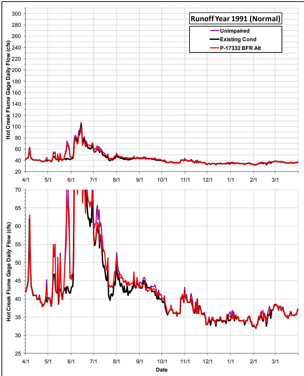
Daily Flows (cfs) at the USGS Hot Creek Flume Gage under the Permit 17332 Bypass Flow Requirements Alternative, the Existing Condition and the Index of Unimpaired Conditions during Runoff Year 1991
