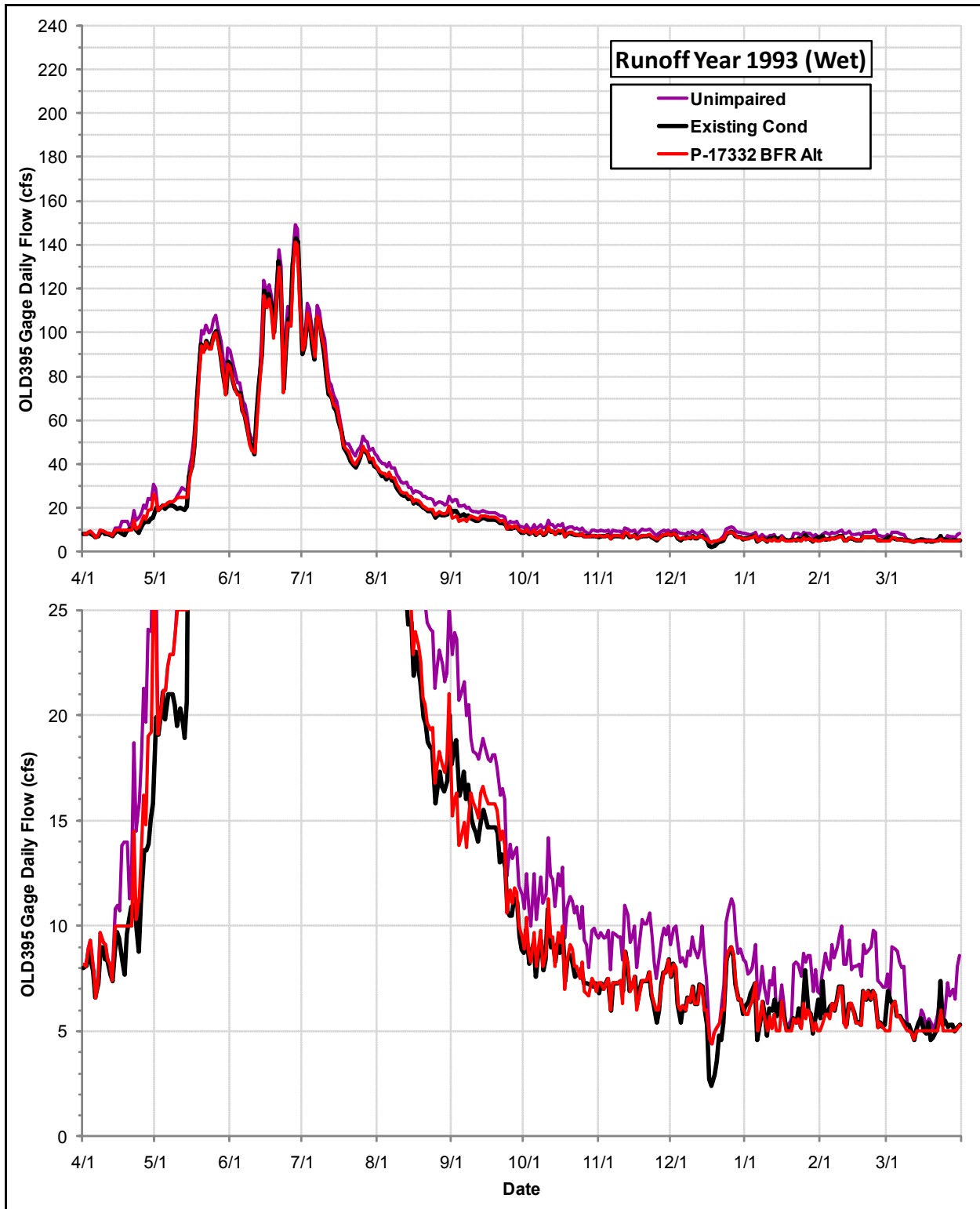
Daily Flows (cfs) at the OLD395 Gage under the Permit 17332 Bypass Flow Requirements Alternative, the Existing Condition and the Index of Unimpaired Conditions during Runoff Year 1993
