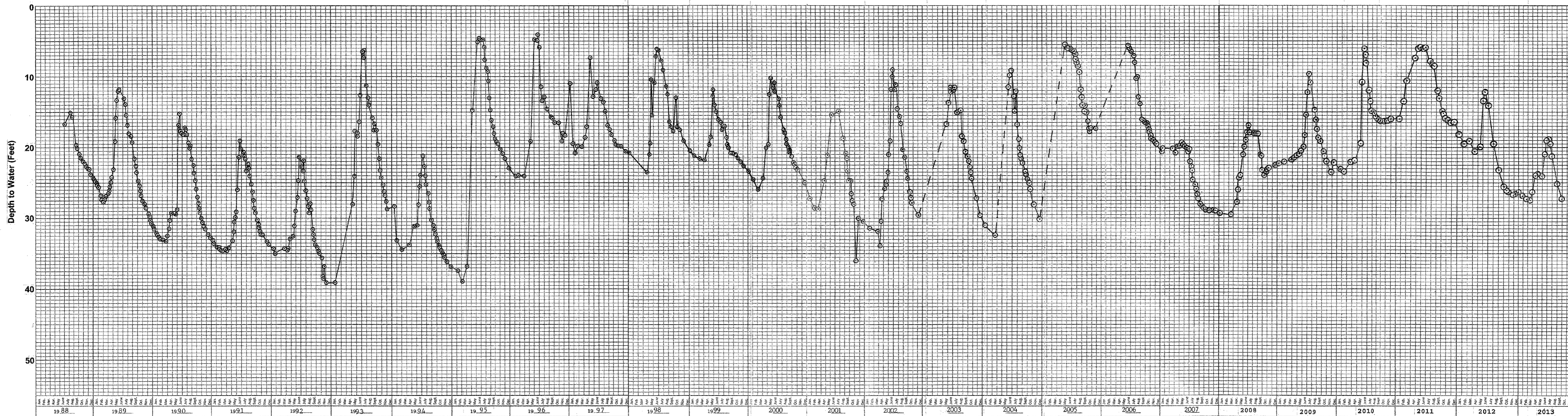
WATER-LEVEL HYDROGRAPH FOR WELL NO. 11M
