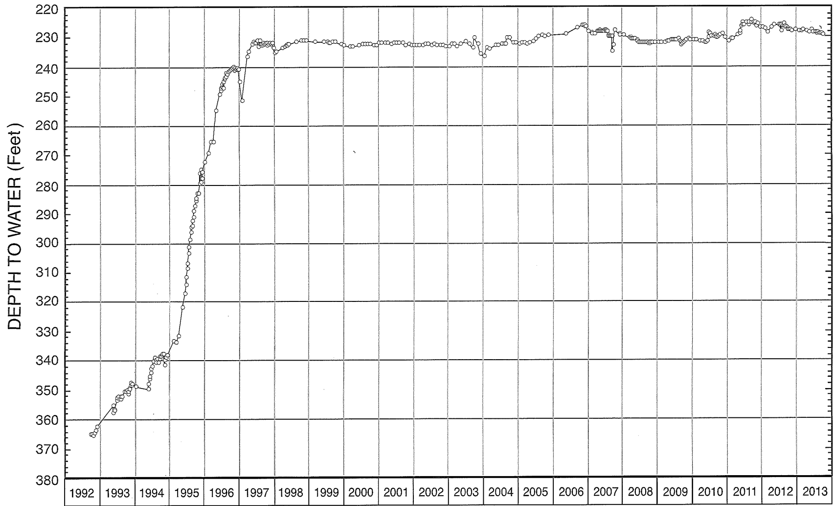
FIGURE 10 - WATER-LEVEL HYDROGRAPH FOR WELL NO. 21
