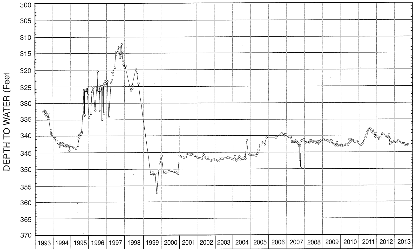
FIGURE 9 - WATER-LEVEL HYDROGRAPH FOR WELL NO. 19
