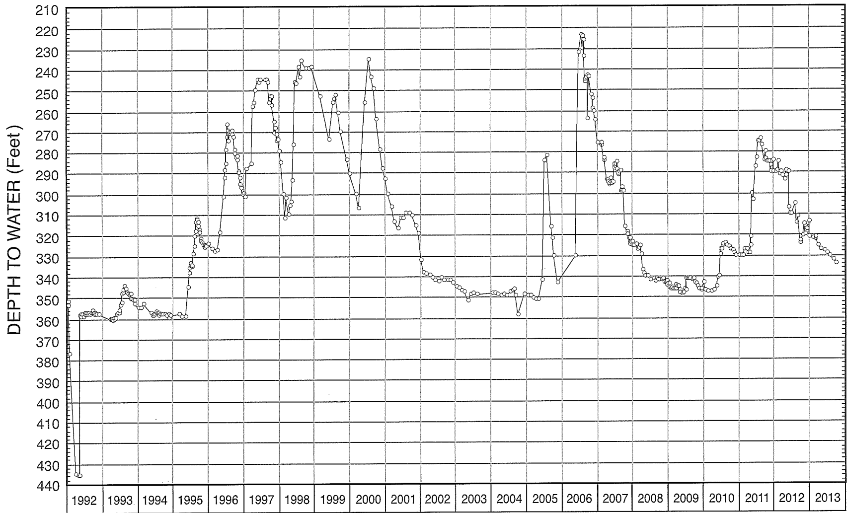
FIGURE 8 - WATER-LEVEL HYDROGRAPH FOR WELL NO. 14M
