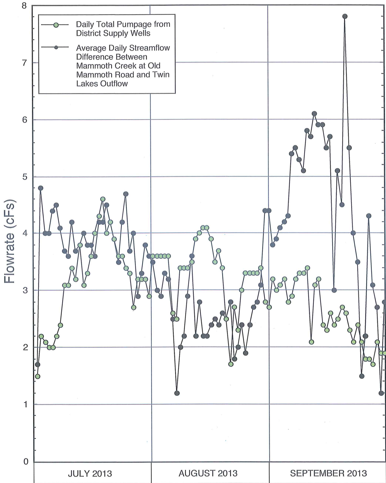
FIGURE 21 - RELATIONSHIP BETWEEN MAMMOTH CREEK STREAMFLOW AND TWIN LAKES OUTFLOW DIFFERENCE, AND DISTRICT PUMPAGE (JULY-SEPTEMBER 2013)
