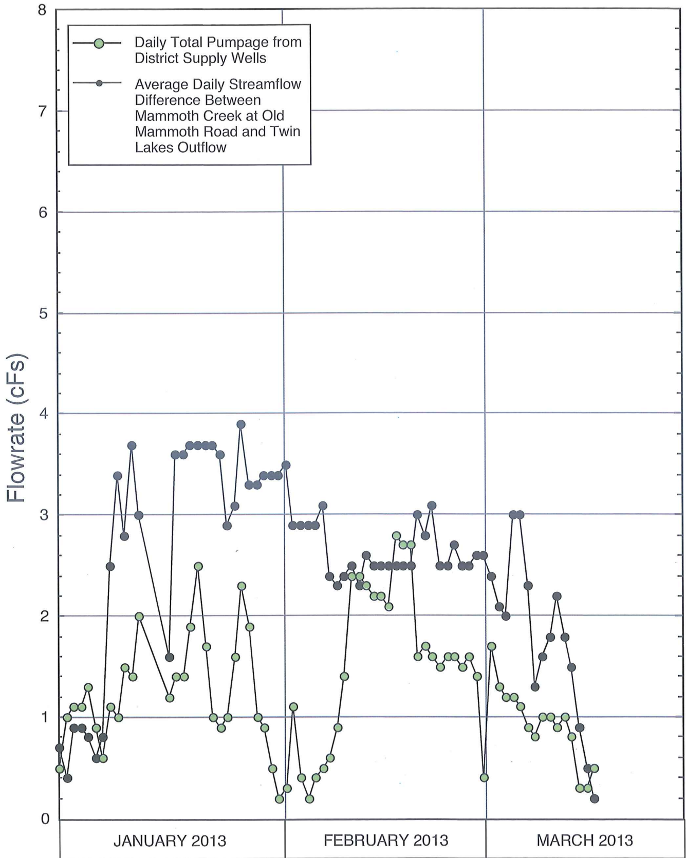
FIGURE 20 - RELATIONSHIP BETWEEN MAMMOTH CREEK STREAMFLOW AND TWIN LAKES OUTFLOW DIFFERENCE, AND DISTRICT PUMPAGE (JANUARY-MARCH 2013)
