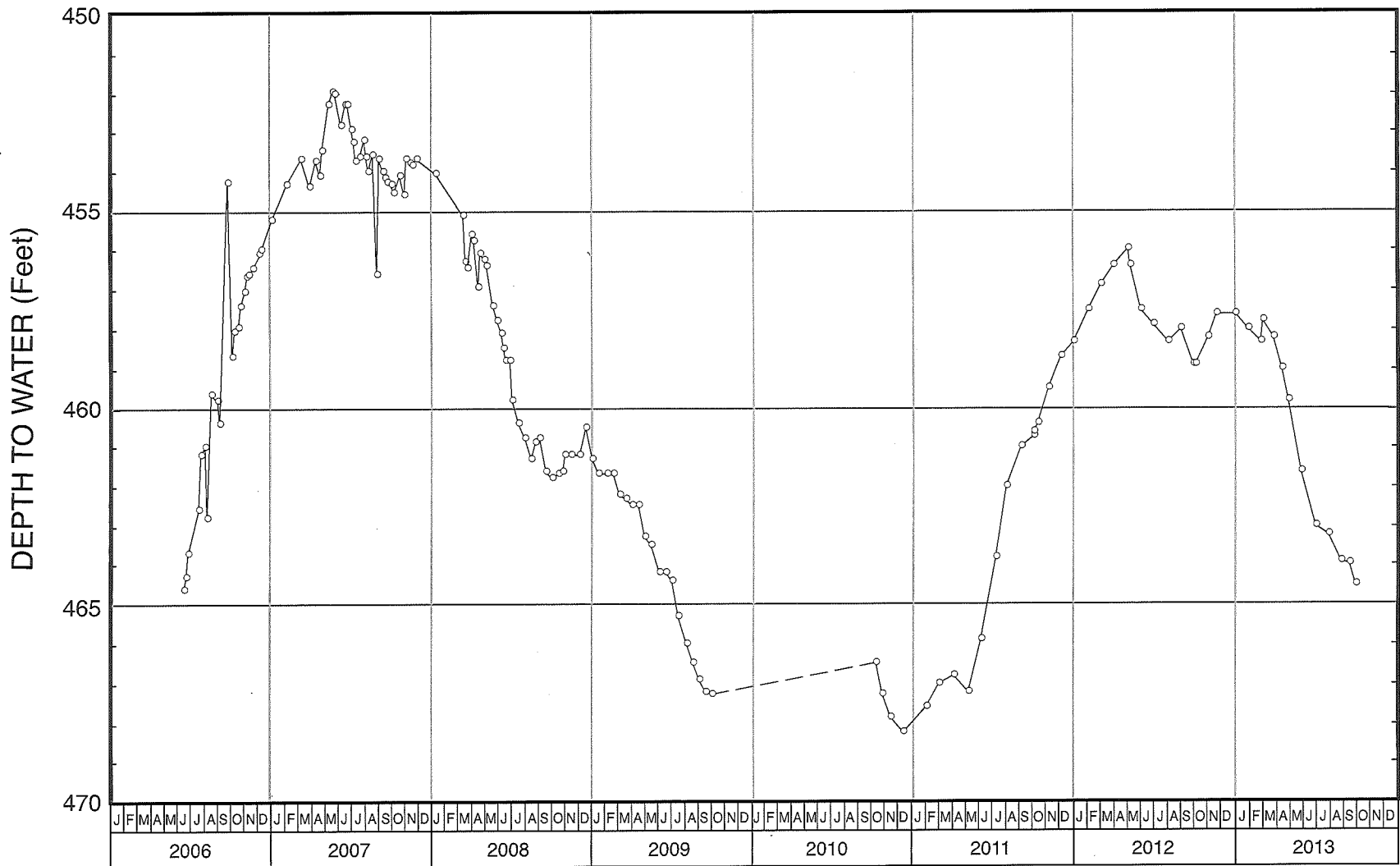
WATER-LEVEL HYDROGRAPH FOR WELL NO. 30
