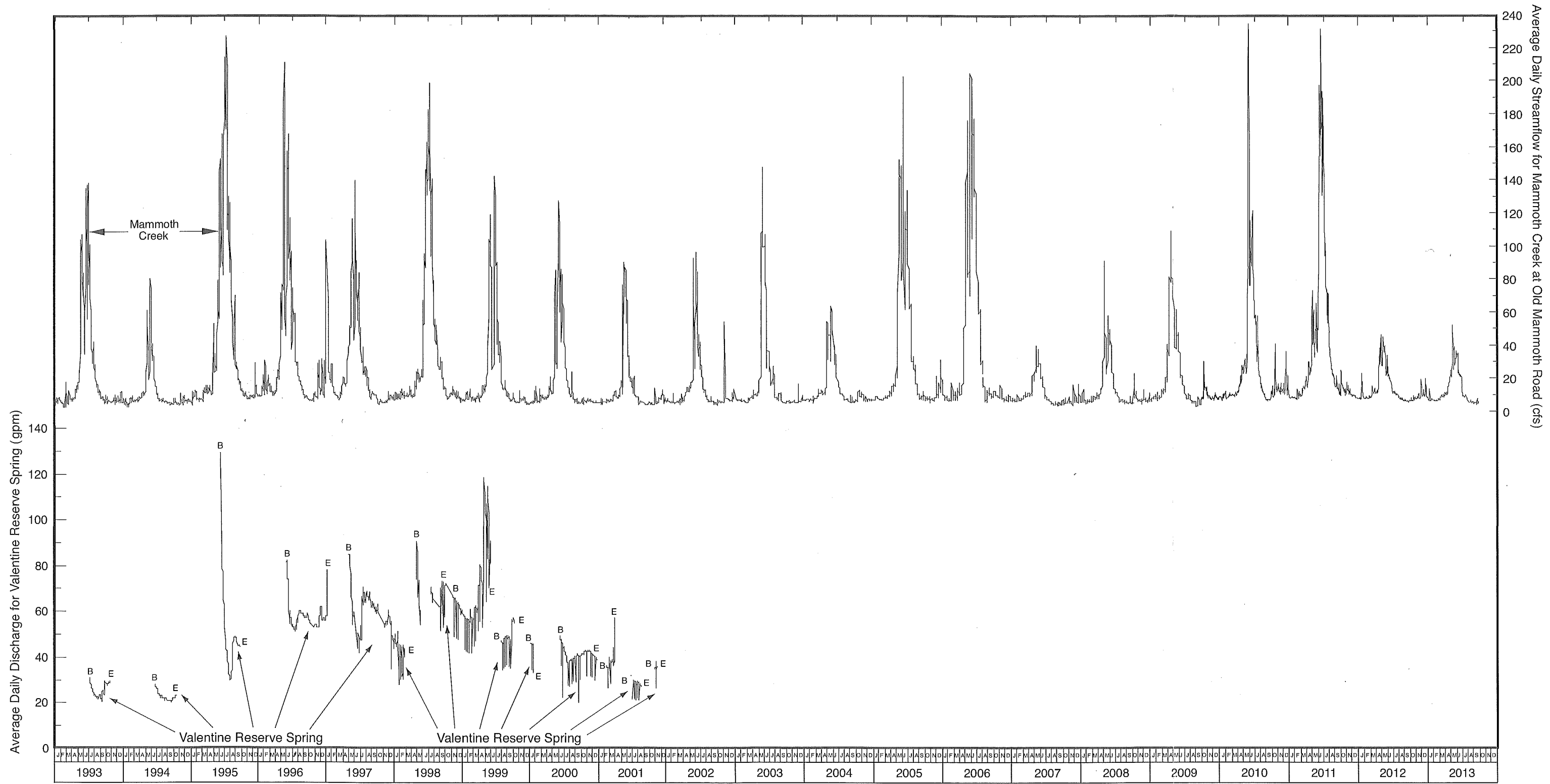
FIGURE 22- FLOW FOR VALENTINE SPRING (1993-2001) AND MAMMOTH CREEK STREAMFLOW (1993-2013)
