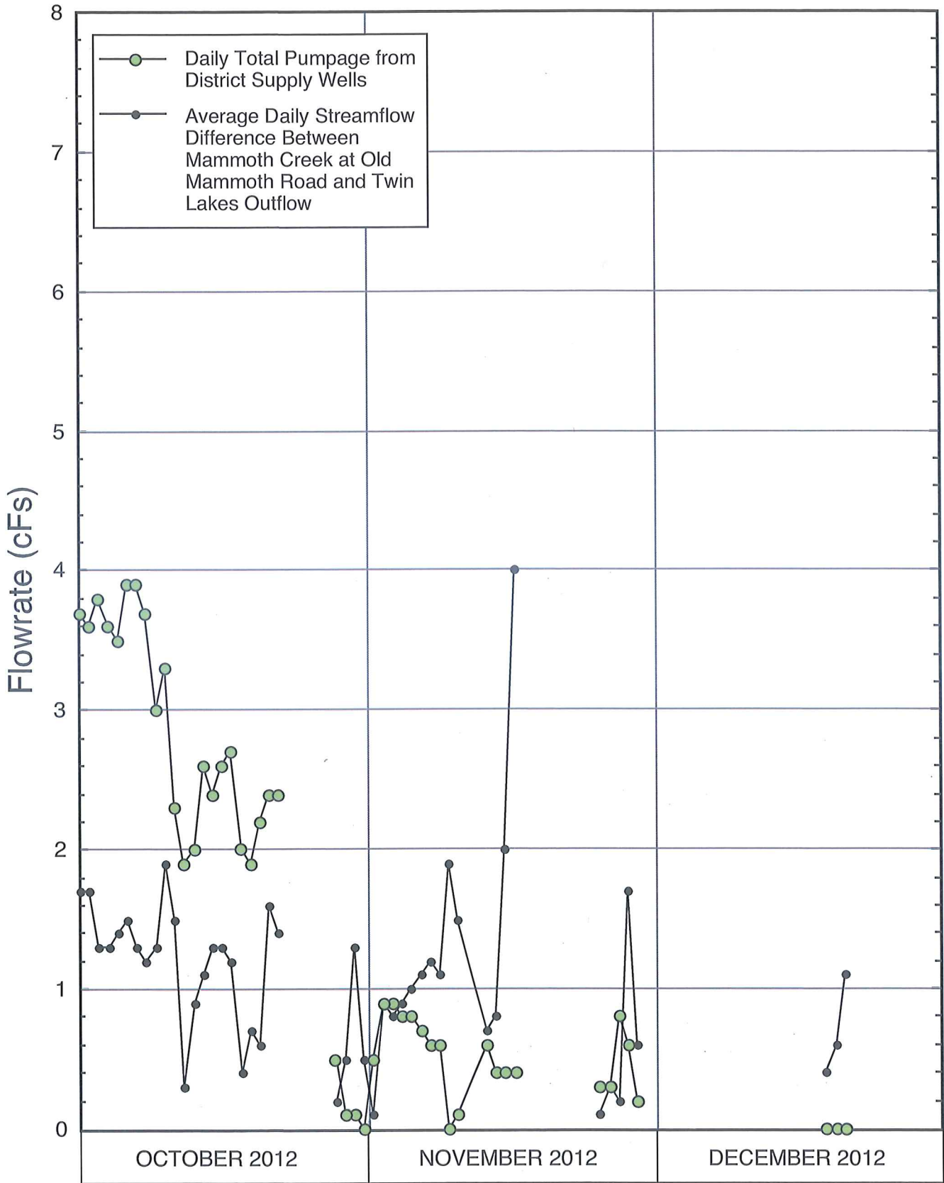
FIGURE 19 - RELATIONSHIP BETWEEN MAMMOTH CREEK STREAMFLOW AND TWIN LAKES OUTFLOW DIFFERENCE, AND DISTRICT PUMPAGE (OCTOBER-DECEMBER 2012)
