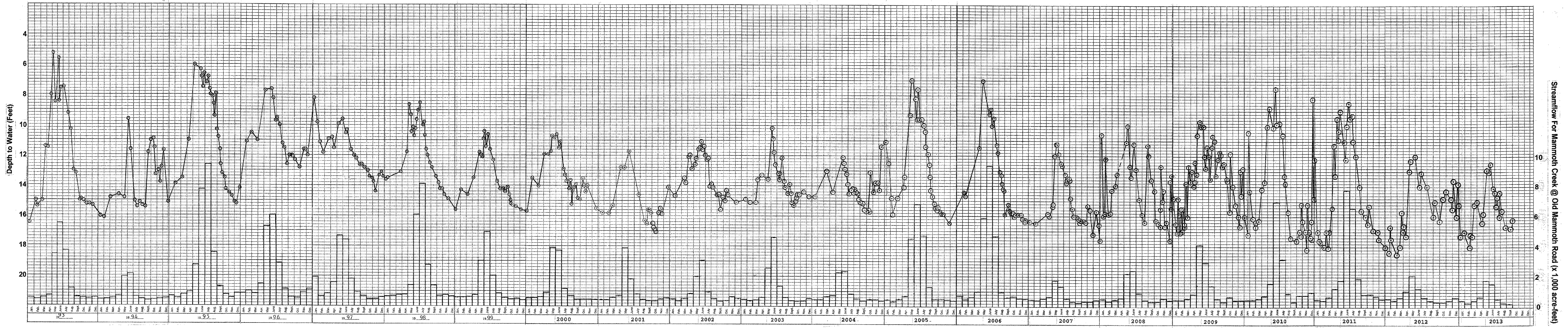
FIGURE 17-WATER-LEVEL HYDROGRAPH FOR WELL NO. 23 AND MAMMOTH CREEK STREAMFLOW
