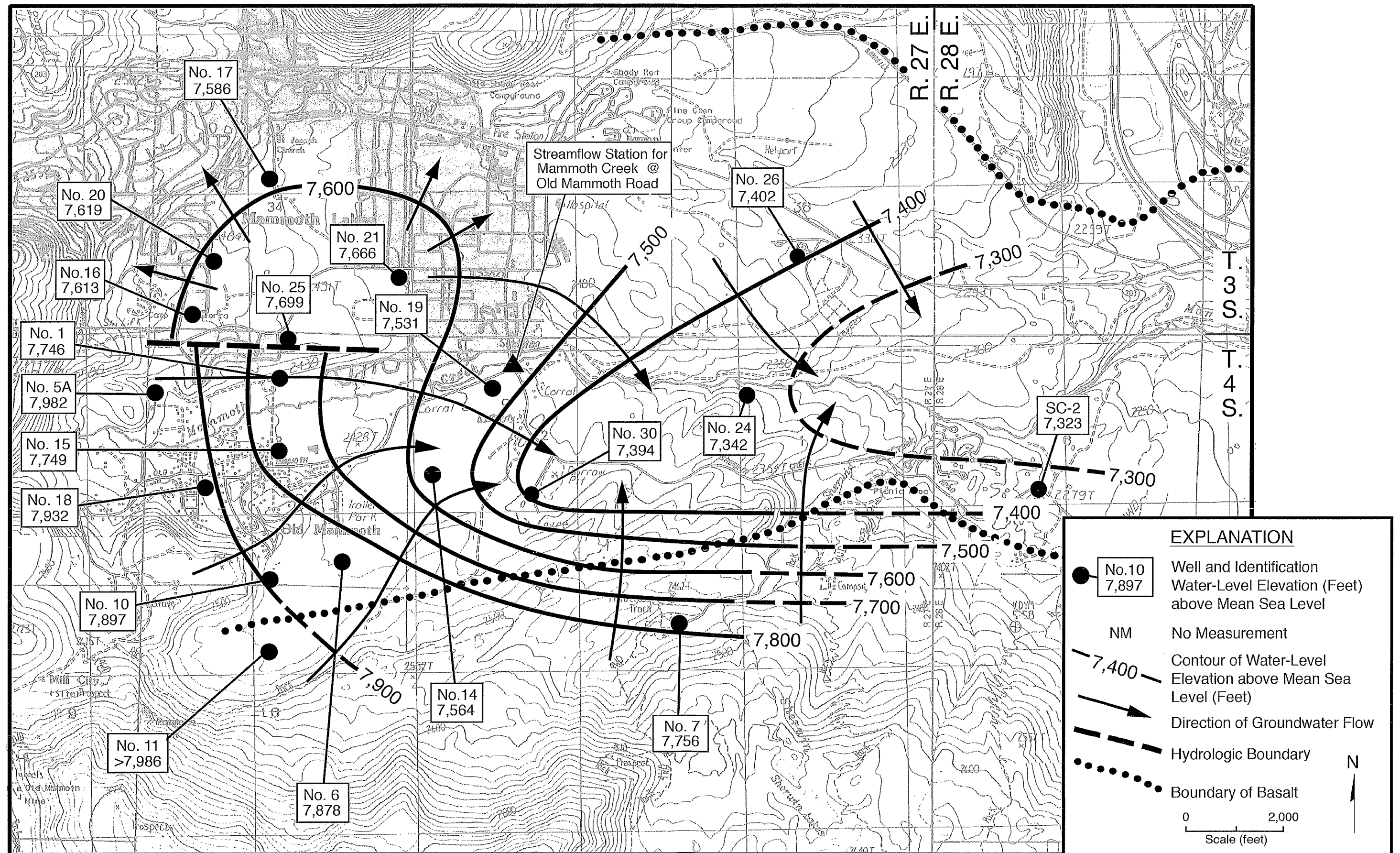
FIGURE 21 - WATER-LEVEL ELEVATIONS IN LATE SEPTEMBER 2020
