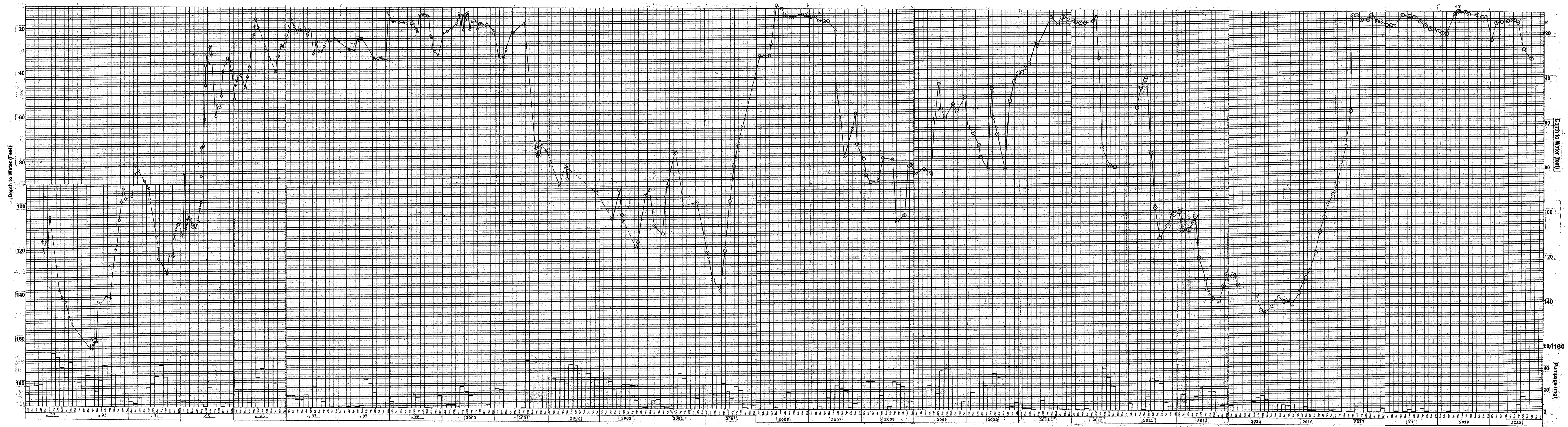
WATER-LEVEL AND PUMPAGE HYDROGRAPH FOR WELL NO. 10
