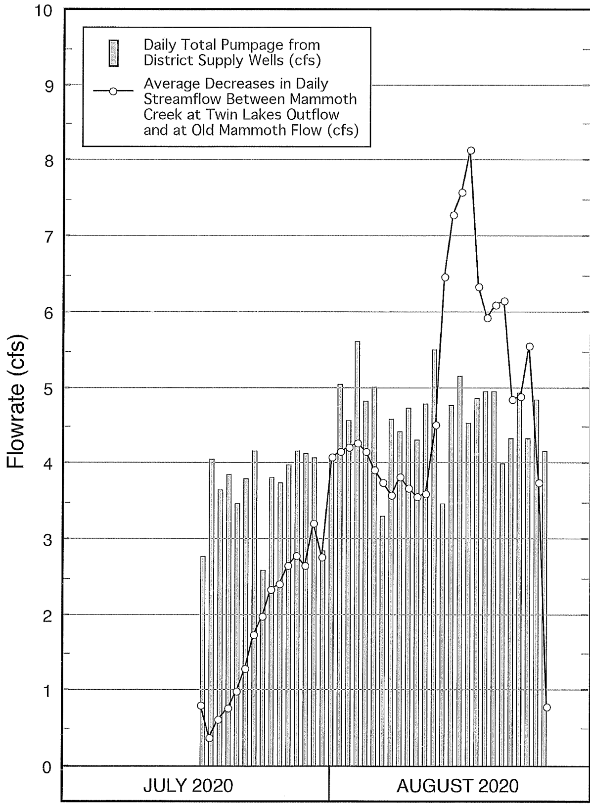
FIGURE 22 - RELATIONSHIP BETWEEN DIFFERENCE IN MAMMOTH CREEK STREAMFLOW AT TWIN LAKES OUTFLOW AND OLD MAMMOTH ROAD AND DISTRICT SUPPLY WELL PUMPAGE (JULY - AUGUST 2020)
