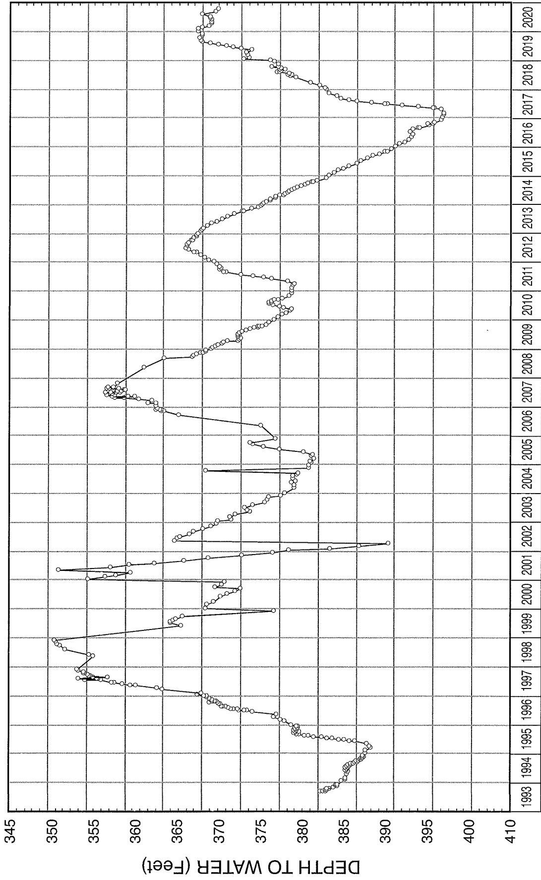
FIGURE 12 - WATER-LEVEL HYDROGRAPH FOR WELL NO. 24
